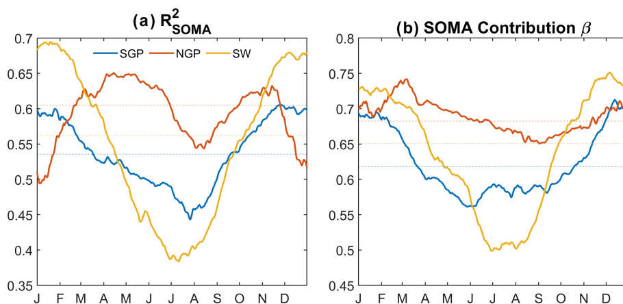
Figure 5. (a) Seasonal variation in the percentage of P' variance explained by P'_{SOMA} ( R^2_{SOMA} ) for the three regions; each data point is calculated within a 91 d calendar window. Thin dashed lines represent the value for all year round. (b) Same as (a) but for seasonal variation in the percentage of moist circulation (SOMA) contribution determined by fitting a simple linear regression model between P'_{SOMA} and P' during a 91 d calendar window ( P'_{SOMA} = \beta P' ).
