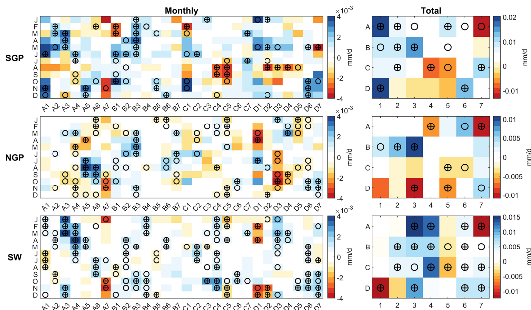
Figure 9. Frequency-weighted P'_{SOMA} difference between positive and negative PDO phases (monthly PDO index > 0.5 and < -0.5 ) for different nodes in different months. For each row or month, nodes marked with a circle (with a plus sign) indicate that the frequency differences are significant positive or negative at the 0.10 (0.05) level, and they can be considered PDO-related nodes for that month.
