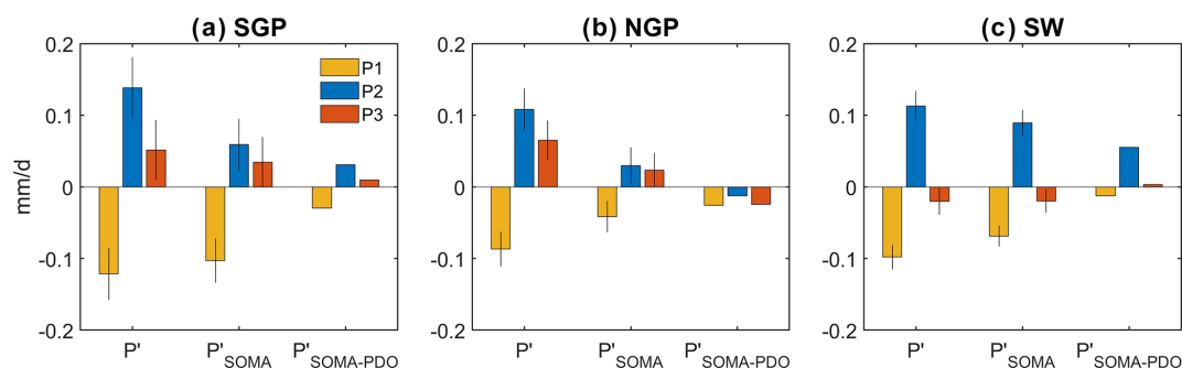
Figure 8. Mean P' , P'_{SOMA} , and P'_{SOMA-PDO} during three periods with shifting PDO phases (P1: 1950–1976; P2: 1977–1998; P3: 1999–2021) in the three regions (a) SGP, (b) NGP, and (c) SW. Error bars in (a) and (b) represent the 95 % confidence intervals of the mean P' and P'_{SOMA} .
