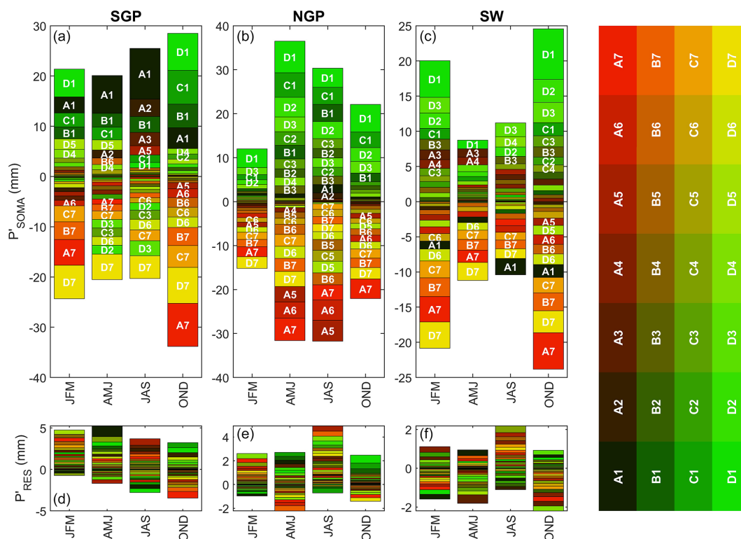
Figure 7. Average moist circulation contribution (SOMA; a–c) and residual (RES; d–f) to P' from each node in each 3-month season (January–March, April–June, July–September, and October–December) over each region (SGP, NGP, SW). The colors of nodes are assigned in such a manner that adjacent nodes exhibit greater similarity in color compared to nodes that are farther apart.
