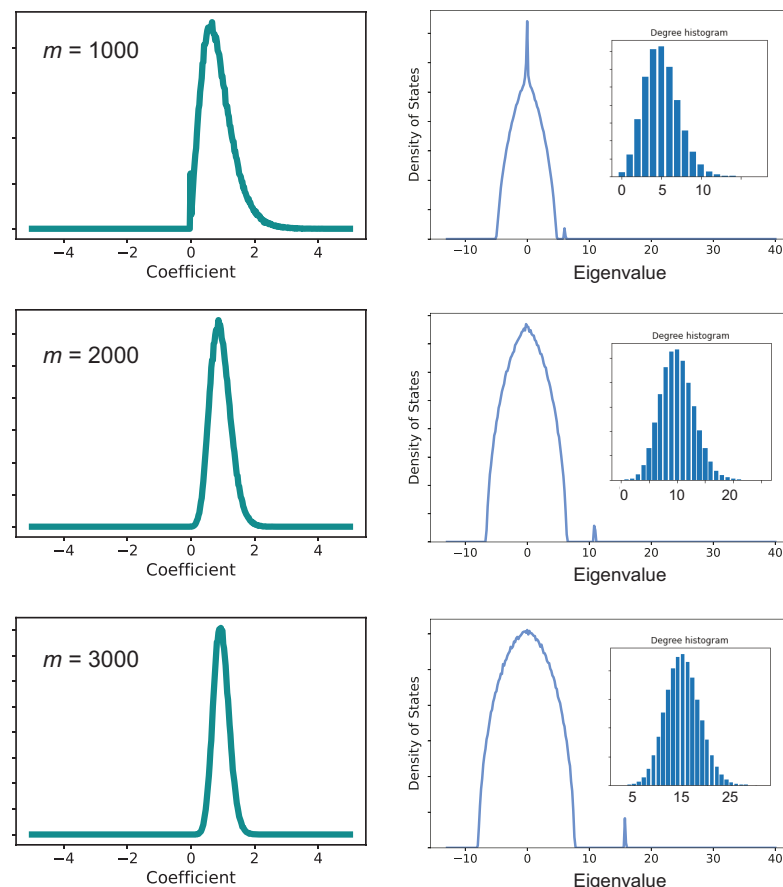
Figure 3. Data from calculations for n = 400 and k = 80 with various values of m , as indicated. The left panels plot the distribution of eigenvector coefficients, normalized such that the emergent state has an eigenvector (1, 1, 1, \dots) . Notice that the emergent state becomes dominant for large values of m . The right panels show the spectrum of the eigenvalues. The emergent state splits off from the semi-circle distribution to higher eigenvalues. The inset panels show the distribution of degree at the graph vertices.
