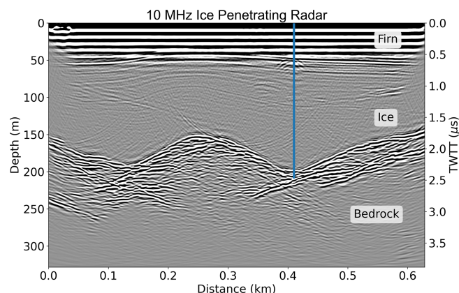
Figure 2. Ground-penetrating radar profile collected with 10 MHz BSI radar across the Begguya plateau in 2022. Standard processing techniques were applied to the data using ImpDAR (Lilien et al., 2020). The two-way travel time (TWTT) is plotted on the y axis on the right side. The Denali ice core drilling (DEN-13B) is indicated by the vertical blue line.
