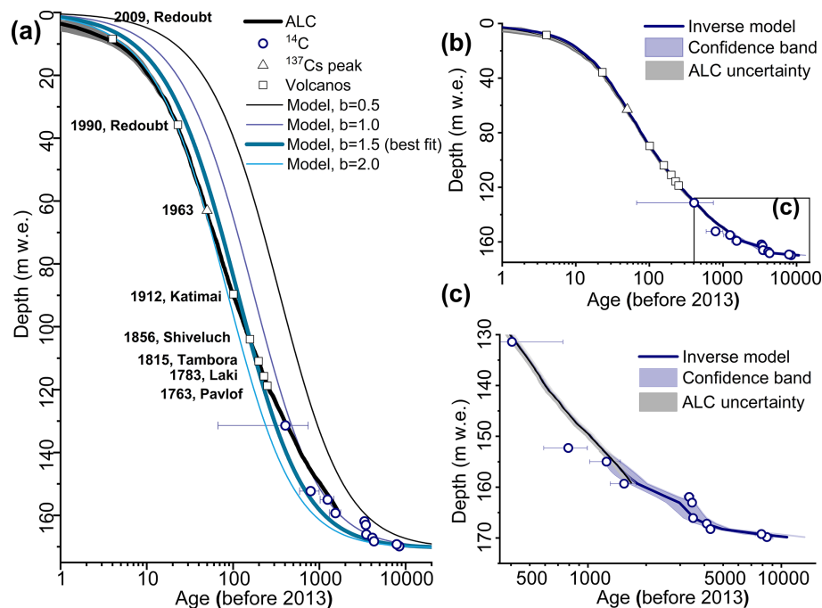
Figure 4. Denali ice core (DEN-13B): annual layer counting (ALC), dating horizons ( ^{14}\text{C} , volcanos, ^{137}\text{Cs} peak), and modeled, continuous age–depth relationship (1D ice flow model; see main text). (a) Model output for constant accumulation rates ( b , in \text{m w.e. yr}^{-1} ). (b) Modeled age–depth relationship for variable b (inverse model). (c) Zoom of the deepest part. All error bars indicate the 1\sigma uncertainty.
