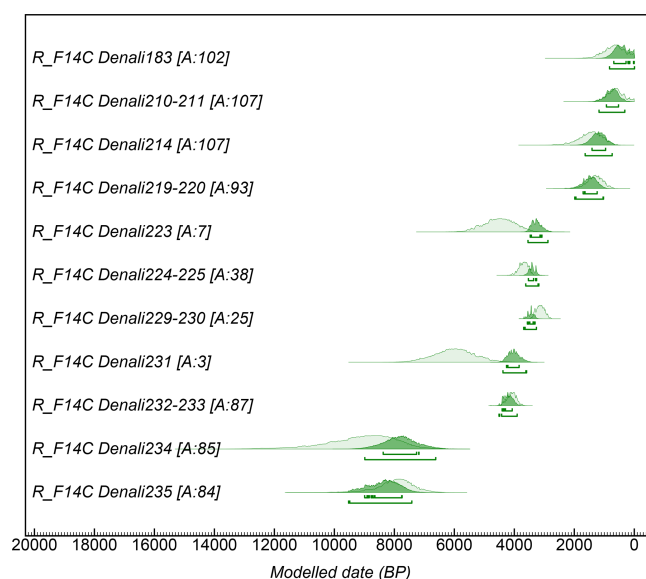
Figure 3. Calibrated ^{14}\text{C} age probability distributions for samples from the Denali ice core (DEN-13B), as derived in OxCal v4.4.4 using the IntCal 20 radiocarbon calibration curve (Ramsey, 2021; Reimer et al., 2020). Light green areas indicate the a priori age probabilities and the dark green areas the a posteriori probabilities when sequential ordering of samples is assumed (see main text). The agreement index ( A ) indicates overlap between these two probability functions. A value < 60 indicates poor agreement (see main text). The 1\sigma and 2\sigma range is indicated by the lines below the probability distribution areas.
