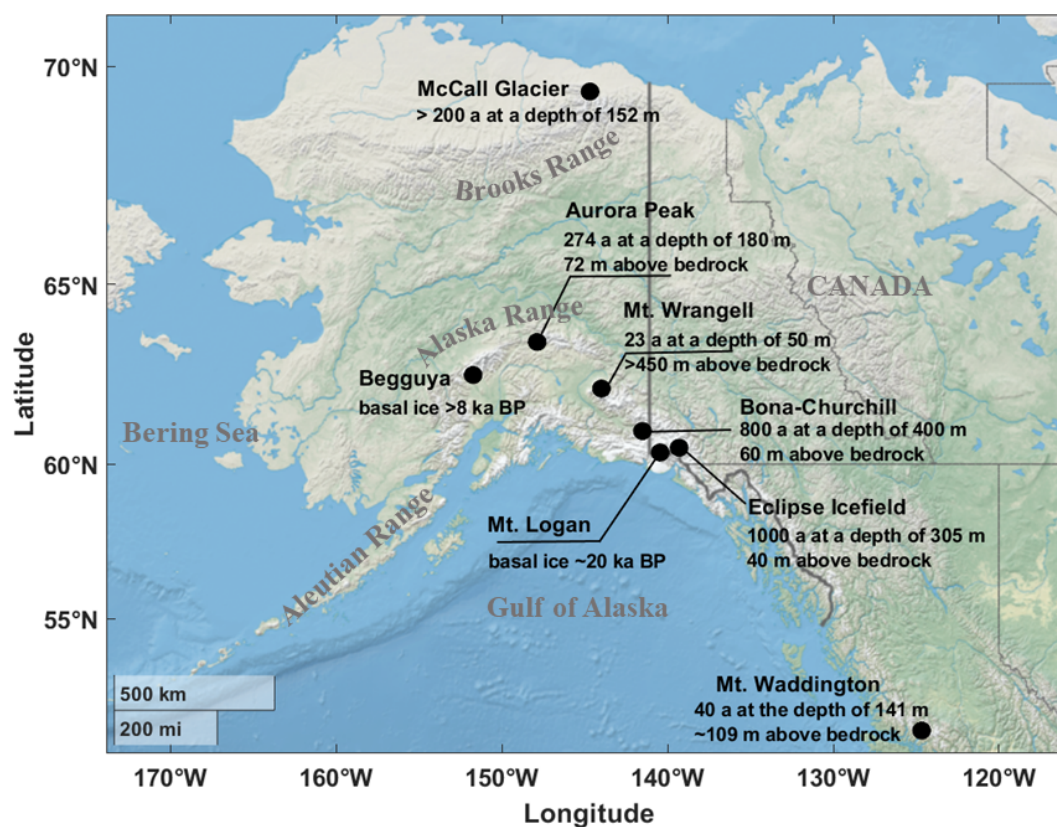
Figure 1. Location map of North Pacific ice core sites and the age of the oldest ice dated from each location: Begguya (Mt. Hunter; this study), McCall Glacier (Klein et al., 2016), Aurora Peak (Tsushima, 2015), Mt. Wrangell (Yasunari et al., 2007), Bona-Churchill (Porter et al., 2019), Mt. Logan (Fisher et al., 2008), Eclipse Icefield (Yalcin et al., 2007), and Mt. Waddington (Neff et al., 2012).
