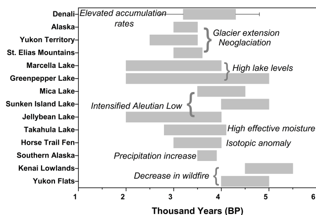
Figure 5. Regional paleoclimate changes as reported in previous studies (Anderson et al., 2005a, b, 2006, 2016, 2019; Broadman et al., 2020; Clegg and Hu, 2010; Denton and Karlén, 1977; Heusser et al., 1985; Jones et al., 2019; Kelly et al., 2013; Schiff et al., 2009; Solomina et al., 2015) and the period of elevated annual net accumulation rates indicated in the Denali ice core DEN-13B (this study; see main text).
