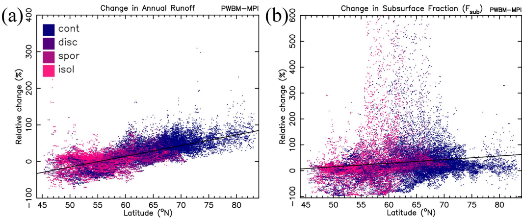
Figure 7. Change in (a) annual total runoff (%) and (b) F_{sub} , with grid cell latitude from the PWBM-MPI simulation for all pan-Arctic domain grid cells. Colors indicate permafrost classification (continuous, discontinuous, sporadic, or isolated) for the cell from the IPA dataset (Fig. 1c).
