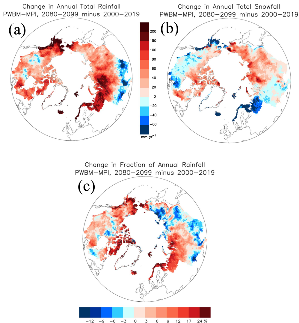
Figure 3. Change in (a) annual rainfall ( \text{mm yr}^{-1} ), (b) annual snowfall ( \text{mm yr}^{-1} ), and (c) the fraction of rainfall to total precipitation from the PWBM-MPI simulation.
