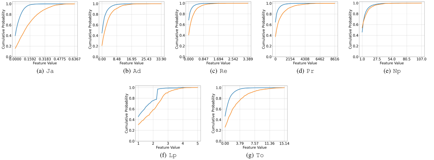
Fig. 4. Cumulative distribution functions (CDFs) for each of the seven feature vectors from s_{20} . CDFs of non-formed links are marked in blue, and CDFs of formed links are shown in orange. These demonstrate that there is (a) an observable difference in distribution between the two populations for each feature and (b) an inverse relationship between number of shortest paths and shortest path length.
