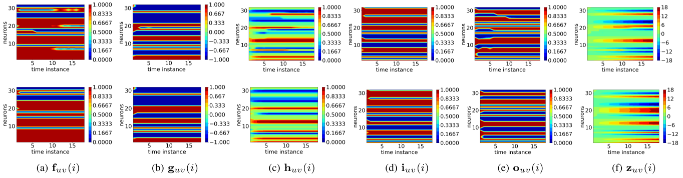
Fig. 7. Neuron activations of each gate \mathbf{f}_{uv}(i) , \mathbf{g}_{uv}(i) , \mathbf{h}_{uv}(i) , \mathbf{i}_{uv}(i) , \mathbf{o}_{uv}(i) , and \mathbf{z}_{uv}(i) over time of the LSTM layer inside the CRNN model for two particular links (u, v) in algo . The fact that several gate dimensions are non-zero indicates that information is propagating across multiple time periods for prediction. The top row demonstrates activations for a link formed late in the course, and the bottom row demonstrates activations for an early-formed link.
