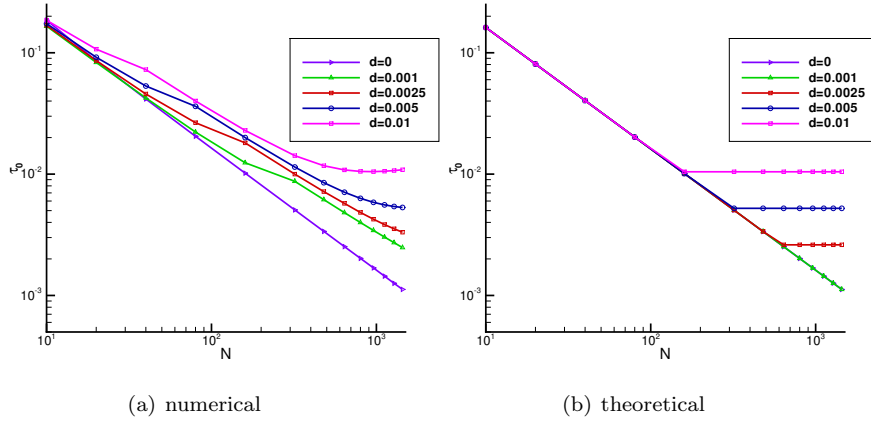
FIGURE 6. The maximal value of time step to ensure monotonicity stability for scheme IMEX(3,4,3)-LDG(2). (a) numerical; (b) theoretical by Fourier analysis.
