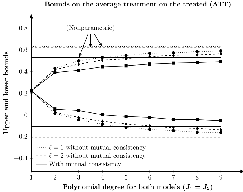
Fig. 4. Imposing mutual consistency tightens bounds on the average treatment on the treated (ATT) for both parametric and nonparametric specifications of the MTR functions.
