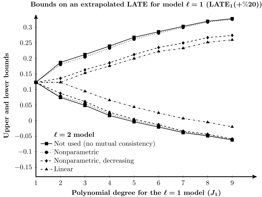
Fig. 5. The \ell = 2 model provides identifying content for parameters, such as \text{LATE}_1(+\%20) , that can only be defined using the \ell = 1 model.
