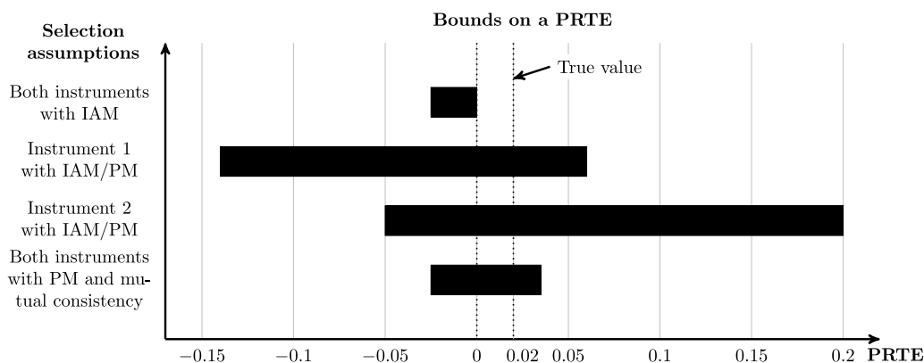
Fig. 6. Bounds on the PRTE of shifting \frac{1}{4} mass from Z = (1, 0) to Z = (0, 1) .
