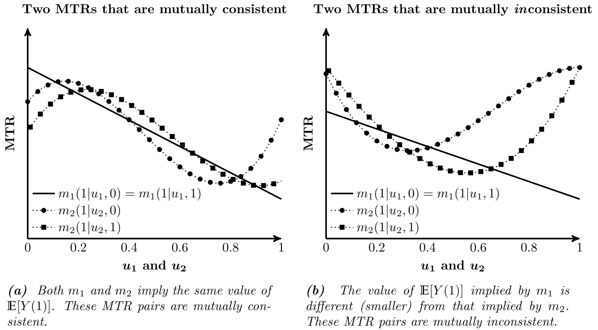
Fig. 2. MTRs along different margins of selection (different U_\ell ) are not directly comparable. Nevertheless, they are not completely unrelated, since both MTRs provide a description of the entire population.
