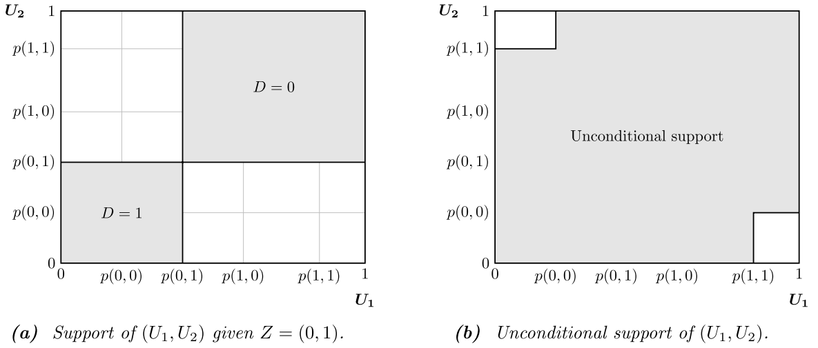
Fig. 1. The joint support of (U_1, U_2) when L = 2 and Z = \{0, 1\}^2 . While both U_1 and U_2 have uniform marginal distributions over [0, 1] by construction, their joint support will be a proper subset of the unit square conditional on Z . If Z has finite support, as in this example, then the unconditional support of U will also be a proper subset of the unit square.
