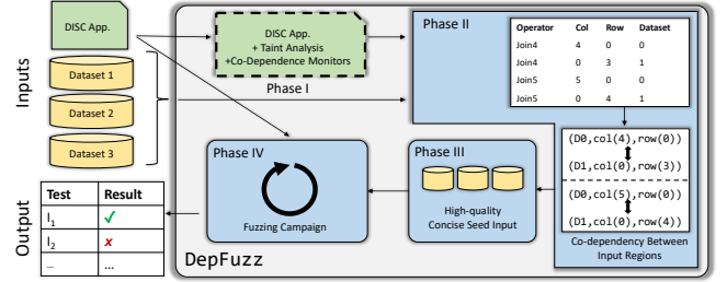
Figure 4: Workflow of DEPFAZZ.
