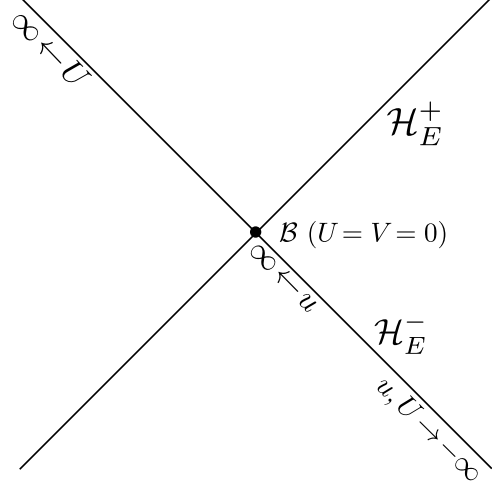
FIG. 4. Bifurcate Killing horizon
