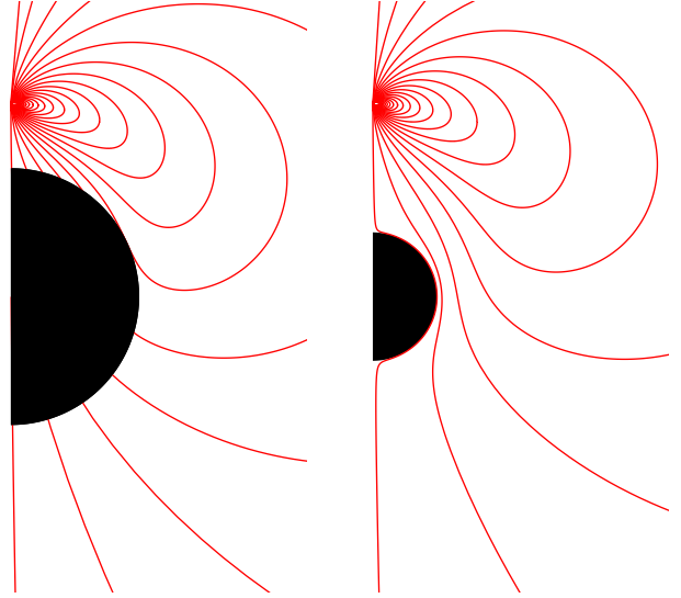
FIG. 3. If a charge q is placed in a spatial superposition of proper separation d , the “which path information” is contained in the difference of the Coulomb fields, which is field of a dipole p = qd . Here we show the electric field lines (level sets of electric flux through a surface of revolution) for a dipole at r_0 = 3M on the symmetry axis of a non-rotating (left) and maximally rotating (right) Kerr black hole. (The black hole region r < M + \sqrt{M^2 - a^2} is shown in black.) In the extremal case, the field does not penetrate inside (the black hole Meissner effect), and correspondingly there is no horizon-induced decoherence.
