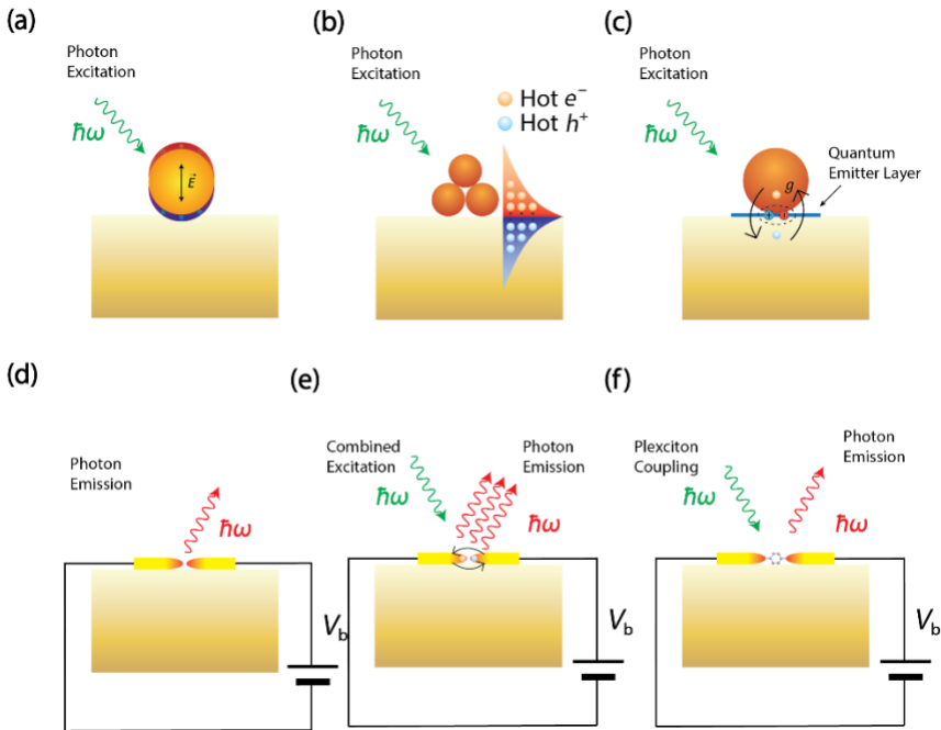
Figure 1 Optically or electrically driven plasmonic nanostructures. (a) Photon excitation induced electrical field enhancement inside a nanoparticle (Purcell effect). (b) Photon excitation induced hot carrier generation in plasmonic nanostructures. (c) Plasmon-exciton coupling probed through optical excitation. (d) Electrically driven plasmonic tunnel junction for light emission. (e) Combined electrical and optical excitation for enhanced hot carrier induced light emission. (f) Combined excitation for probing plexciton strong coupling in molecular scale plasmonic systems.
