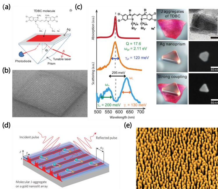
Figure 10 Experimental platforms for plexciton coupling. (a) Schematic representation of Kretschmann configuration, where the momentum of the incident light has been increased by the prism to obtain polaritonic dispersion curves [206]. (b) SEM image of hole array in a silver film fabricated through focus ion beam milling [207]. (c) The coupling between metallic nanoparticle plasmons and molecule excitons probed by extinction, scattering spectroscopy and electron microscopy. Spectra with various coupling strength are shown in the left [213]. (a)-(c) are reproduced with permission from the American Physical Society. (d) A hybrid nanostructure consisting of a 50 nm thick film of J-aggregate molecules in a polymer matrix on a gold nano slit array for coherent ultrafast spectroscopy [208]. Reproduced with permission from the Springer Nature Group. (e) False colour SEM image of an ensemble of aligned Au nanorods supported by a transport substrate [210]. Reproduced with permission from the American Chemical Society.
