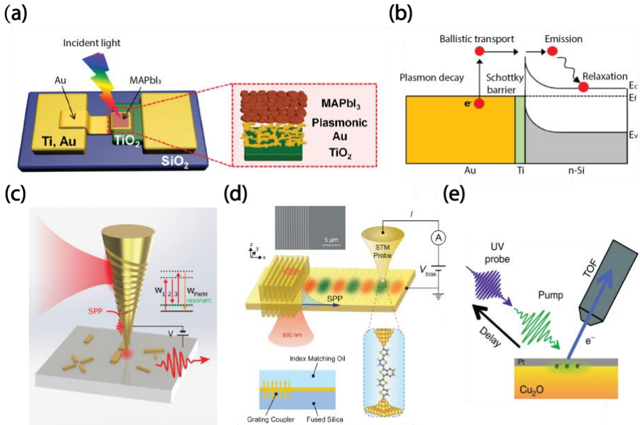
Figure 3 Experimental techniques for hot carrier detection and imaging. (a) Illustration of the MAPbI 3 /Au/TiO 2 nanodiode configuration. The inner structure can be seen in the enlarged view of the active area [93]. Reproduced with permission from the American Chemical Society. (b) A plasmon-induced hot electron can undergo ballistic transport to the Schottky barrier interface, leading to the tunnelling into the semiconductor[96]. Reproduced with permission from the American Chemical Society. (c) A pair of femtosecond pulses of variable time delay are grating coupled and focused at an STM apex, which can be used as an ultrafast nanoimaging tool [112]. Reproduced with permission from Springer Nature Group. (d) The hot carrier distribution induced by the propagating SPPs from the grating is mapped by the single molecule junction based on the STM probe [119]. Reproduced with permission from American Association for the Advancement of Science. (e) A schematic illustration depicts the application of time-resolved two-photon photoemission spectroscopy to Cu 2 O [122]. Reproduced with permission from Springer Nature Group.
