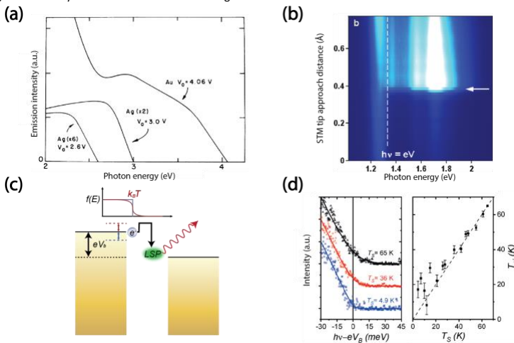
Figure 4 Below-threshold light emission in plasmonic nanostructures due to inelastic electron tunnelling and thermally broadening induced overbias emission (a) Light emission spectra from electrically biased Au and Ag tunnel junction at 77 K, an energy cutoff equal to the applied bias can be clearly seen [18]. (b) Light emission spectra map from a biased STM junction when varying the tip surface distance [147]. (c) An electron can gain excess energy from the thermal broadening of the Fermi-Dirac distribution, creating a higher energy LSP which leads to the overbias emission [148]. (a)–(c) are reproduced with permission from the American Physical Society. (d) Electronic temperatures obtained from fitting the tail at the energy cutoff position of the spectral data, plotted together with the junction temperature in the right panel [160]. Reproduced with permission from the Springer Nature Group.
