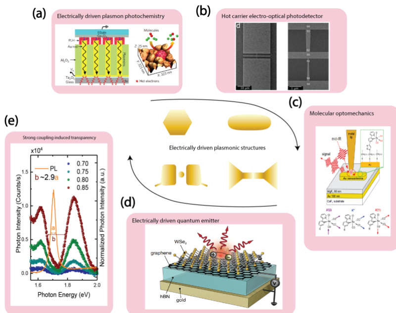
Figure 13 Prospective research topics based on electrically driven plasmonic processes. (a) Electrically driven plasmonic nanorod used as reactive tunnel junction [302]. Reproduced with permission from the Springer Nature Group. (b) Plasmonic-active asymmetric gold nanostructures for photodetectors [271]. Reproduced with permission from the American Chemical Society. (c) Antenna-coupled vibrational spectroscopy based on STM [230]. Reproduced with permission from the National Academy of Science. (d) Hybrid plasmon-exciton coupling system as a quantum emitter [260]. (e) A coupled single molecular junction based on STM shows transparency in the light emission spectra [246]. Reproduced with permission from the Springer Nature Group.
