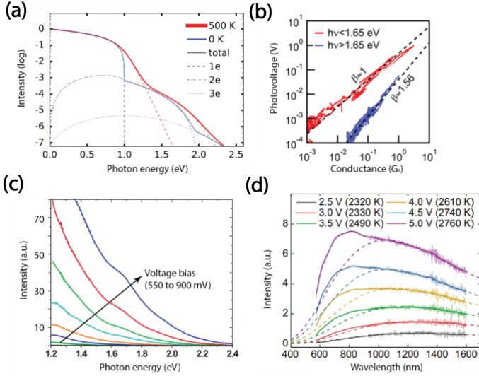
Figure 6 Experimental results for multielectron tunnelling and blackbody-like light emission. (a) Calculated light emission spectra of multielectron cotunnelling processes at T=0 and 500 K. Contributions from 1e, 2e and 3e processes are indicated by dashed, dash-dotted and dotted lines, respectively. The sharp turns occurring at 1e, 2e, and 3e position are smeared out at elevated temperatures[146]. Reproduced with permission from the American Physical Society. (b) Traces of measured photovoltage (proportional to the emission intensity) versus the STM junction conductance for both below- and above-threshold emission[166]. Reproduced with permission from the American Chemical Society. (c) Emission spectra from a planar electromigrated junction, with giant overbias emission[145]. Reproduced with permission from the American Chemical Society. (d) Emission spectra from a planar graphene tunnel contact, which resemble the blackbody radiation spectra (dashed line) but with an added spectral weight[170]. Reproduced with permission from the American Physical Society.
