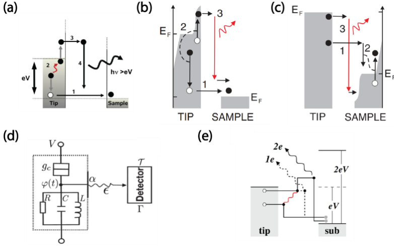
Figure 5 Multielectron coherent tunnelling induced above-threshold light emission (a) Illustration of the hot-hole mechanism producing the 2e light emission[147]. (b) A hot hole created by elastic tunnelling below the Fermi level can go through a cascade and produce a high energy electron above Fermi level, which leads to the overbias photon through inelastic tunnelling[162]. (c) A hot electron can tunnel into the sample, where a subsequent cascade process generates hot holes. The electron-hole recombination give rise to the 2e light emission[162]. (d) The effective electromagnetic circuit model describing the light emission process: SPP damping and photon emission is mimicked through a LRC circuit[163]. (e) One and two electron coherent tunnelling for the 1e and 2e light emission[165]. All figures are reproduced with permission from the American Physical Society.
