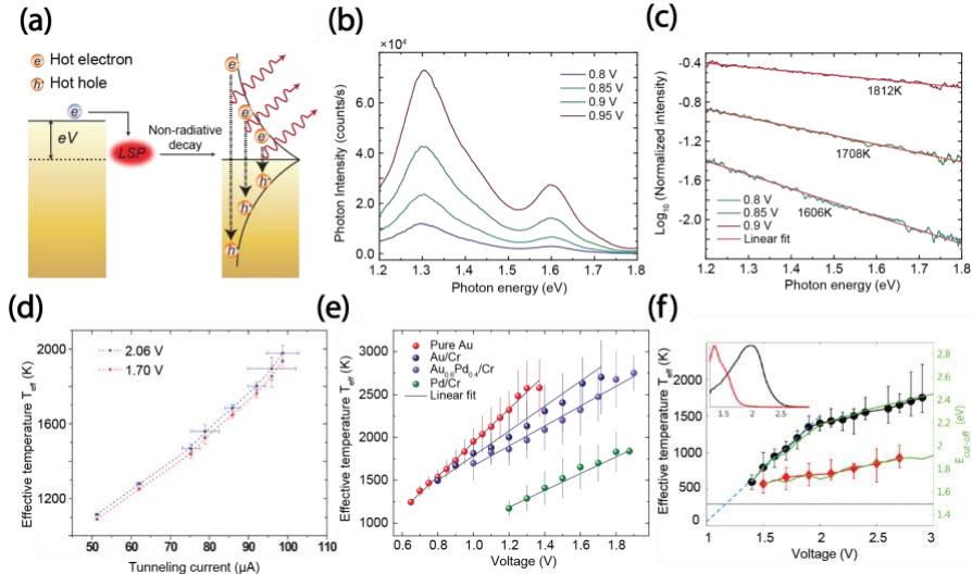
Figure 7 Experimental results for above-threshold light emission due to plasmonic hot carrier recombination. (a) Schematics of above-threshold light emission from plasmon induced hot carrier recombination [92]. (b) Measured light emission spectra under different biases from a planar Au electromigrated junction [92]. (c) Normalization analysis for the data in (b) to extract electron effective temperature through Boltzmann fitting [92]. (d)-(f) Extracted effective temperature from the light emission spectra versus the electrical condition (bias or current). (d) from a blackbody-like hot carrier induced overbias emission [145]. (e) from plasmon induced hot carrier light emission [92]. (f) Similar to (e) but from a vertical metal-semiconductor tunnel junction [174]. All figures are reproduced with permission from the American Chemical Society.
