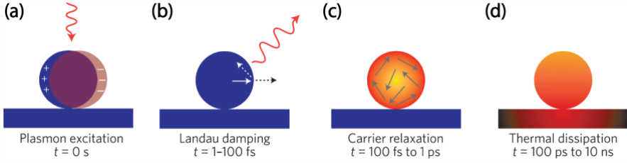
Figure 2 Hot carrier generation and relaxation dynamics. Hot carrier relaxation regimes at different times after initial photon excitation [26]. Reproduced with permission from the Springer Nature group.
