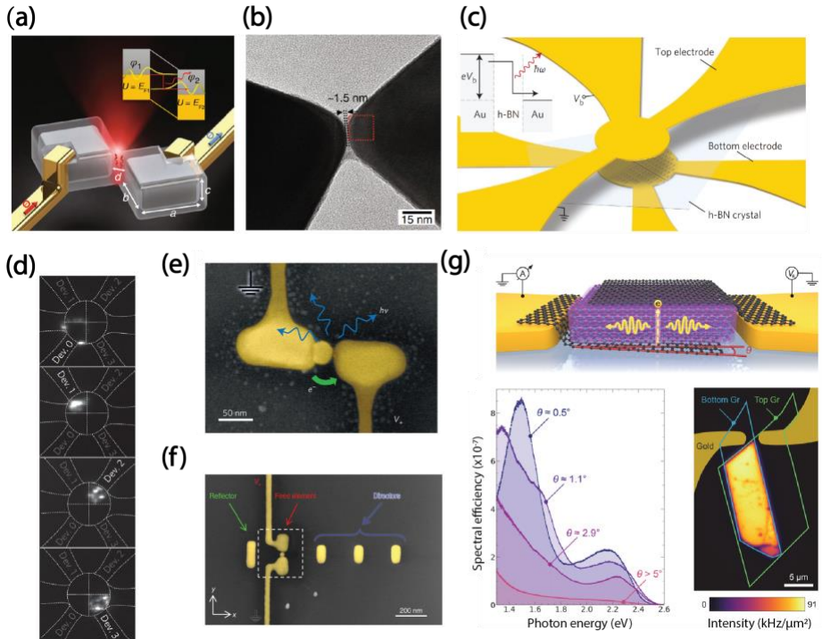
Figure 9 On-chip optoelectronic applications utilizing plasmon-enhanced light emission in molecular scale plasmonic nanostructures. (a) Diagram of a tunnel junction formed by two edge-to-edge Ag single-crystal cubes, with extended electrodes for electrical access [175]. (b) TEM image of the junction structure shown in (a). (c) A vertical tunnel junction structure formed by a few layers of hBN sandwiched between patterned Au electrodes [180]. (d) Images of four light emitting device shown in (c) at a constant applied bias 2.5V. (e) SEM image of a lateral tunnel junction structure consisting of an electrically connected single-crystalline Au nanoantenna sandwiching a Au nanoparticle [177]. (f) SEM image of a Yagi-Uda antenna based on the junction shown in (e), which contains reflector, feed element and three directors [178]. (a)-(f) are reproduced with permission from the Springer Nature Group. (g) Schematic of a twisted Gr/hBN/Gr tunnel junction for electroluminescence. Different spectra from various twisted angle are shown in the bottom left. A false color CCD image of the uniform light emitting area is shown in the bottom right [181]. Reproduced with permission from the American Chemical Society.
