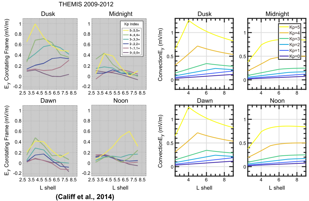
Figure 2. (Left) Radial profiles of the dawn-dusk E -field according to Califf et al. (2014) in the frame corotating with Earth, as a function of L , for select K_p values, in the dusk, midnight, dawn and noon regions, as marked. (Right) Radial profiles of the modified Volland-Stern model convection E -field as a function of L , for select K_p values, and for the same local time regions as the left-hand side panels.
