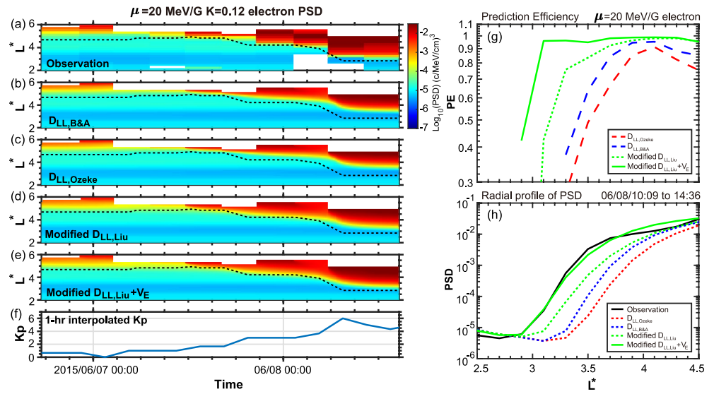
Figure 3. Comparisons between observed and modeled phase space density (PSD) for \mu = 20 MeV/G, K = 0.12 G^{1/2} R_E electrons from 7 to 9 June 2015. (a) PSD calculated from RBSP A&B flux observations; (b) Modeled PSD with D_{LL,B\&A} ; (c) with D_{LL,Ozeke} ; (d) with D_{LL,Liu-mod} ; (e) with D_{LL,Liu-mod} and V_E ; (f) K_p index; (g) prediction efficiency as a function of L^* with different coefficients; (h) PSD radial profile comparisons during the initial enhancement.
