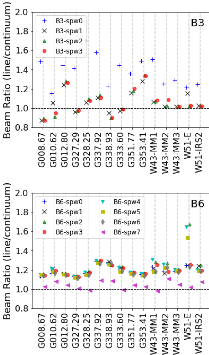
Fig. 5. Ratio of the average line to continuum beam for each protocluster and spectral window (B3 top; B6 bottom panels). Where the average beam is defined as \theta_{\text{ave}} = \sqrt{\theta_{\text{maj}} \times \theta_{\text{min}}} . We scale the ratio linearly to account for the frequency difference between the central frequency of the spectral window and the frequency of the continuum beam. The native beam major and minor axis for each spectral window is listed in Table A.2. The proposed beam and the average recovered continuum beam for all fields are given in Table A.1. The central frequency of the continuum images for B3 and B6 for each protocluster is given in Ginsburg et al. (2022a), and the spectral coverage for each of the line cubes are shown in Table A.3. The dashed horizontal line shows a one-to-one ratio between the line and continuum beams.
