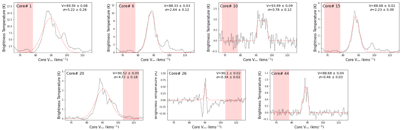
Fig. F.22. Complex-type core-averaged, background-subtracted DCN spectra extracted from the cores in the young protocluster W43-MM2. Readers can refer to Table F.12 for the line fit parameters for each core.
