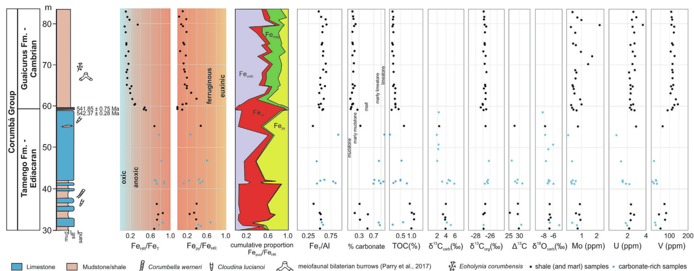
Fig. 3. Chemostratigraphic trends of the Corumbá Group at the Laginha Quarry. Age constraints after Parry et al. (2017). From left to right, geochemical plots represent iron speciation Fe_{HR}/Fe_T and Fe_{Py}/Fe_{HR} ratios (with interpretive thresholds derived from Raiswell et al., 2018), the cumulative proportion of different highly reactive iron pools, Fe_T/Al ratios, the percentage carbonate as determined gravimetrically from acidification, total organic carbon (TOC) weight percent, inorganic and organic carbon isotope ratios as represented by \delta^{13}C_{carb} (‰) and \delta^{13}C_{org} (‰), respectively, the difference between the inorganic and organic carbon isotope ratios represented by \Delta^{13}C , oxygen isotope ratios in the carbonate fraction represented by \delta^{18}O_{carb} (‰) and the relative abundances of redox-sensitive elements molybdenum (Mo), uranium (U) and vanadium (V) in ppm. Enrichment factors and normalizations to TOC or other variables are not presented as most of the concentrations are below or close to typical crustal values, indicating detrital rather than authigenic abundances. Although Parry et al. (2017) described trace fossils at the top of the Tamengo Formation elsewhere, in the Laginha Quarry they only occur at the Guaiçurus Formation. Some of the inorganic carbon and oxygen isotope data are compiled from Ramos et al. (2022), with addition of eight new data points as reported in the Supplementary Data Table S2.
