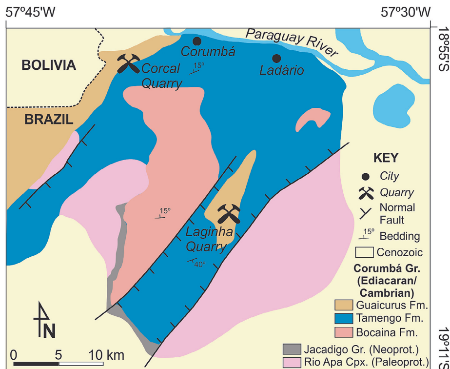
Fig. 2. Simplified geological map of the Corumbá region showing the location of the studied Láginha quarry. For location of the map see Fig. 1. Compiled and modified after Amorim et al. (2020) and Diniz et al. (2021).
