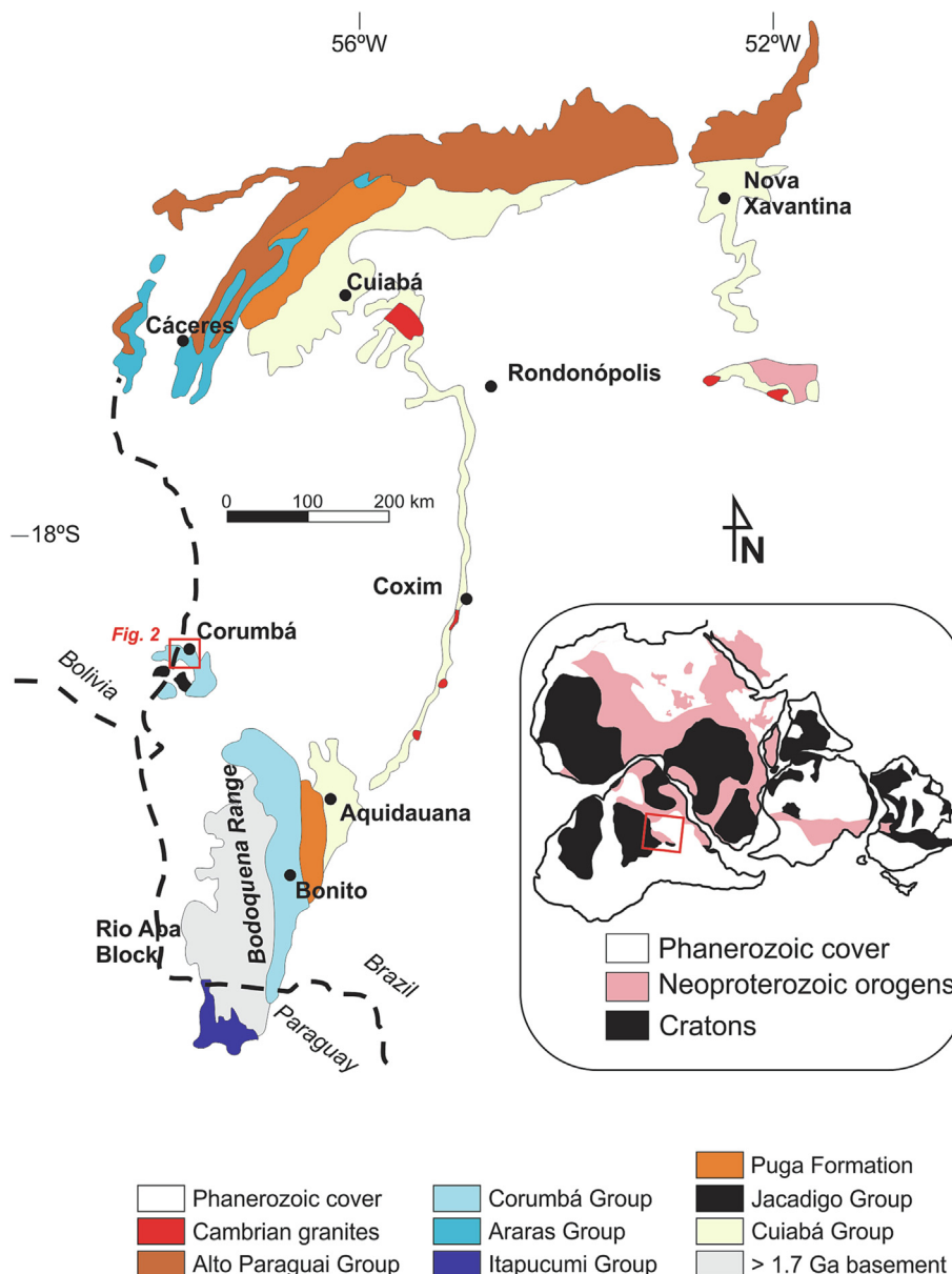
Fig. 1. Schematic geology of the Paraguay Belt in western Brazil. The inset at the bottom right shows the approximate position in western Gondwana. The studied area is marked in the red rectangle. Modified after Caxito et al. (2019). (For interpretation of the references to colour in this figure legend, the reader is referred to the web version of this article.)
