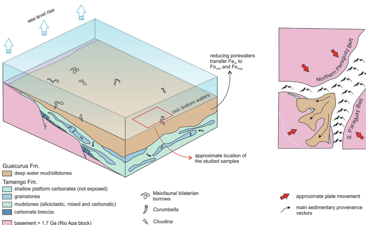
Fig. 4. Models for the deposition of the Tamengo and Guaicurus formations at the Ediacaran–Cambrian transition (left) and tectonic configuration of the basin and adjacent continental blocks (right), with red arrows indicating general movement of the involved paleocontinental blocks and black arrows indicating main sedimentary provenance vectors. The approximate location of the studied samples is indicated by the red rectangles. (A) Deposition of the Tamengo Formation in the late Ediacaran (ca. 550–540 Ma) occurred in a stratified basin with a shallow oxic layer where biomineralizing organisms such as Cloudina and Corumbella thrived. Shell fragments of these were transported down-slope and deposited under ferruginous bottom water conditions. During this time frame, the Amazon, Rio Apa and Paranapanema paleocontinents were rifted apart, and the basin mainly sourced the adjacent Rio Apa block. (B) Deposition of the Guaicurus Formation in the early Cambrian occurred during a major transgression, flooding the basin while the redoxcline was drastically deepened, generating oxic bottom water conditions where bioturbating organisms thrived. Detrital zircon U–Pb age spectra indicates that during this time frame, the basin sourced the mountainous areas related to the Brasiliano Orogen to the west, due to collision of the Amazon, Rio Apa and Paranapanema paleocontinents. (For interpretation of the references to colour in this figure legend, the reader is referred to the web version of this article.)
