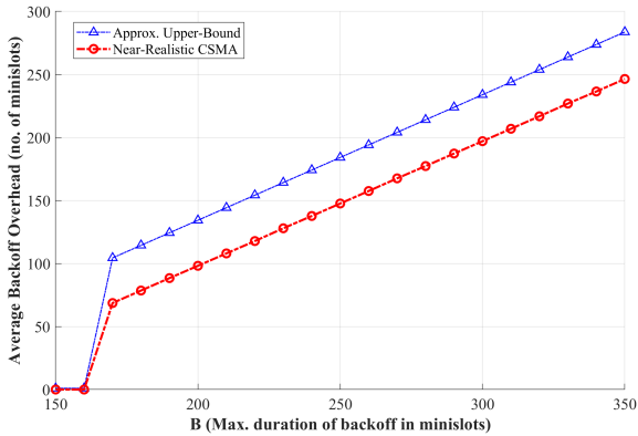
Fig. 9. Average backoff overhead vs. B .
