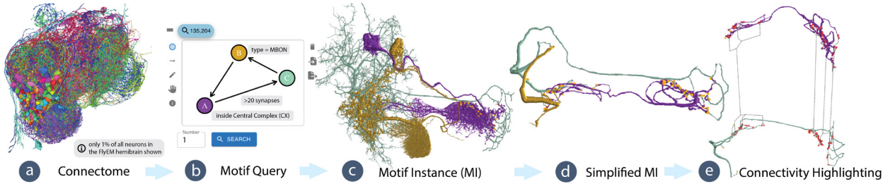
Fig. 1: Visual Motif Analysis. (a) In Vimo , neuroscientists search large brain networks (view online: [29]) by (b) sketching neuronal connectivity motifs. (c) Neurons forming a motif instance (MI) are visualized in 3D. Vimo emphasizes the relationship between the sketched motif and the neurons' connectivity using a continuous focus&context approach (d, e). First, Vimo prunes neuron branches unrelated to the motif (d). Next, users explore the connectivity between neurons in an exploded view that untangles complex neuron morphologies and uses hierarchical synapse clustering and bundling to highlight connections (e). Data: FlyEM Hemibrain [44].
