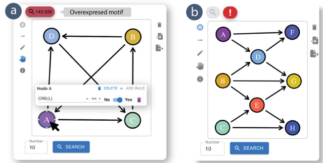
Fig. 6: Motif sketching interface. (a) Users draw nodes and edges of a motif and define biological constraints on the nodes and edges. Additionally, Vimo gives real-time feedback on the absolute count of a sketched motif in the dataset and indicates whether a motif is over- or under-represented in the dataset (red label). (b) When searching the brain network for large motifs, Vimo warns users of potentially long runtimes using a red exclamation mark icon (b - top).
