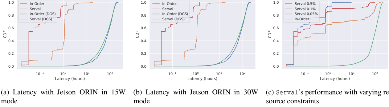
Figure 7: End-to-end latency of Serval compared to in-order baseline. Serval can achieve a median end-to-end latency of 0.1 hours when using distributed ground stations. Serval’s performance is stable across different hardware constraints.
