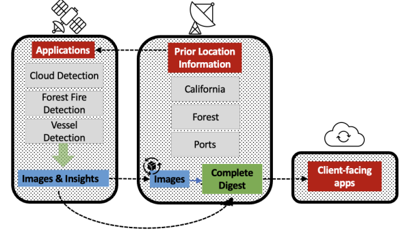
Figure 5: Serval Example Execution: The placement of different compute units for queries defined in Fig. 2.
