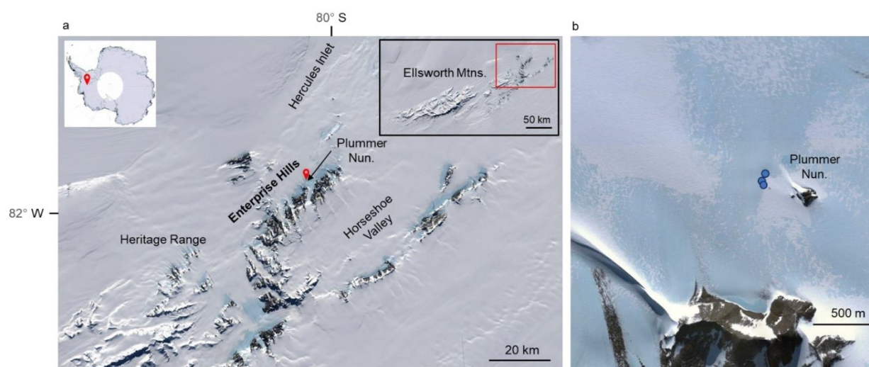
Fig. 5. a) Overview of Enterprise Hills. The red pin indicates the location of Plummer Nunatak. b) Enhanced map showing blue ice area around Plummer Nunatak. Blue dots indicate drill site locations. Base maps for both panels were created from Google Earth: Imagery © 2023 Maxar.
