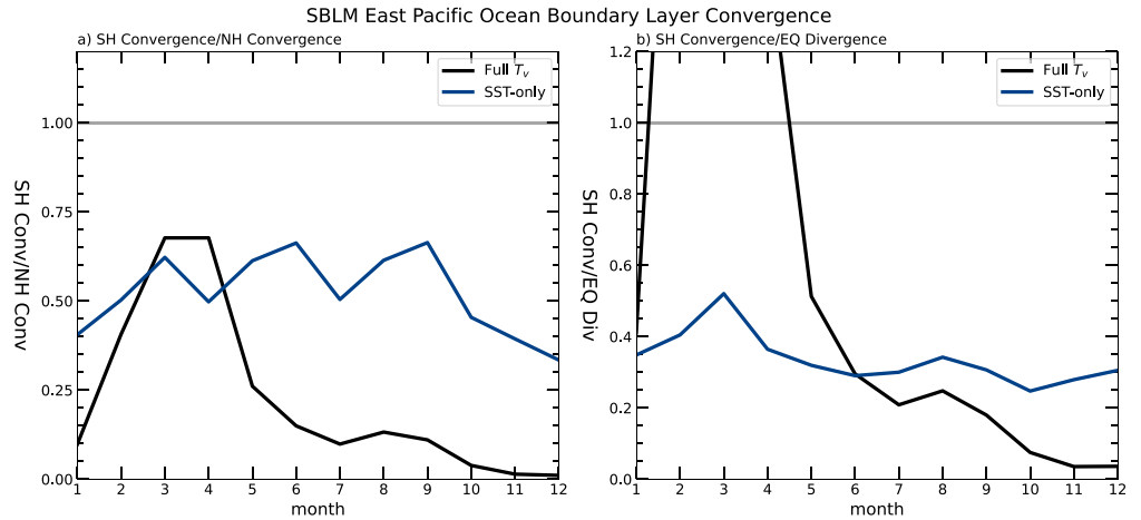
Figure 5. The ratios of the: (a) maxima of NH convergence and SH convergence and (b) maxima of equatorial divergence and SH convergence for the Full T_v PGF (black) and SST-only PGF (blue) SBLM simulations. The SH and NH convergence maxima correspond to the convergence in the gray circles Figures 4a and 4b. The equatorial divergence maxima correspond to the divergence in gray triangles of Figures 4a and 4b.
