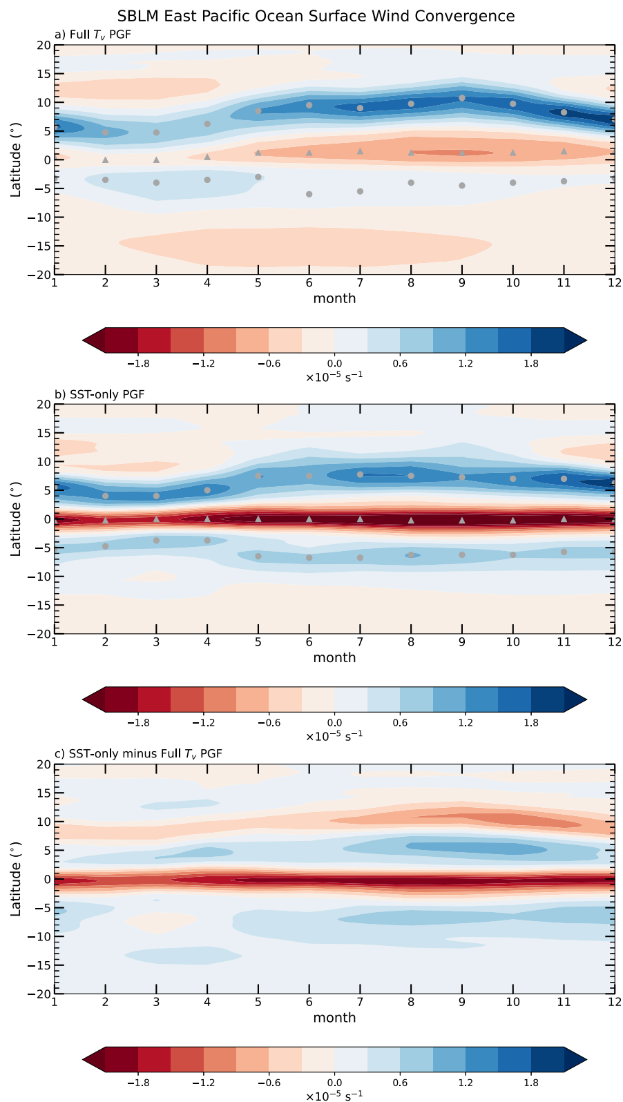
Figure 4. SBLM-simulated surface wind convergence over the east Pacific Ocean ( 90\text{--}125^{\circ}\text{W} ) for the two experiments: (a) Full T_v PGF and (b) SST-only PGF. Panel c shows SST-only minus Full T_v PGF surface wind convergence. In panels a and b, the gray circles are the latitudes of maximum SH and NH convergence and the gray triangles are the latitudes of maximum equatorial divergence.
