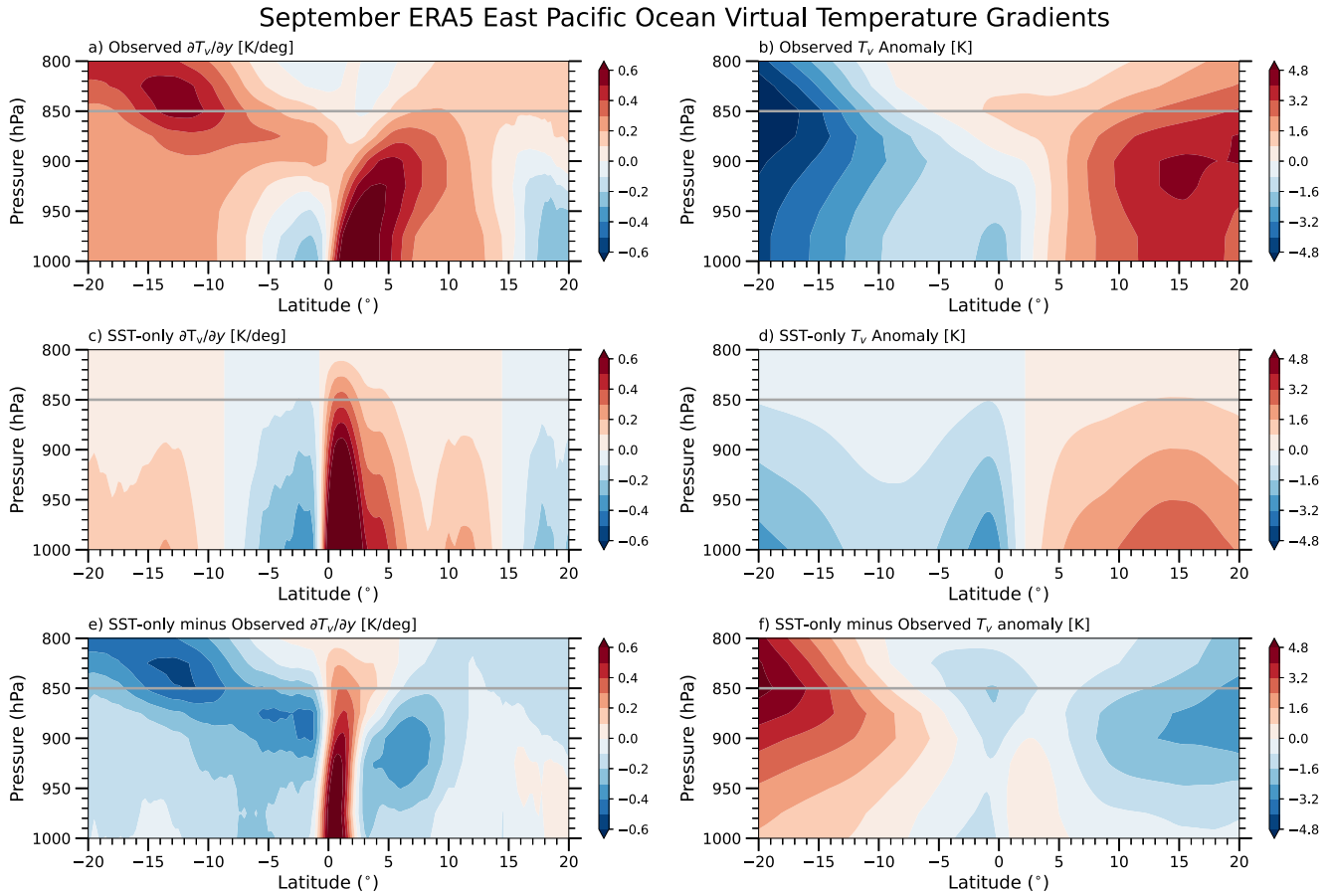
Figure 1. ERA5 meridional T_v gradients and T_v anomalies averaged over the east Pacific Ocean (90–125°W) during September: (a) observed \partial T_v/\partial y , (b) observed T_v anomaly, (c) SST-only \partial T_v/\partial y , (d) SST-only T_v anomaly, (e) SST-only minus observed \partial T_v/\partial y , and (f) SST-only minus observed T_v anomaly. T_v anomalies are relative to the 20°S–20°N mean.
