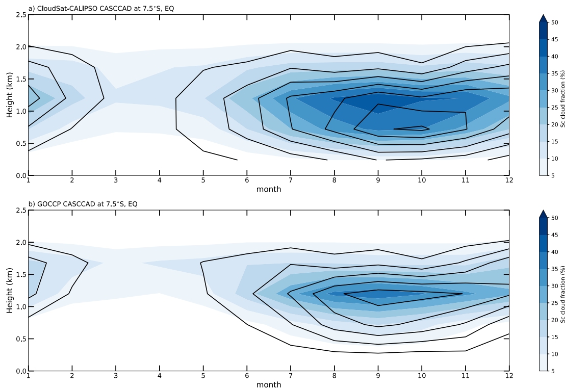
Figure 7. Stratocumulus (Sc) cloud fraction (%) averaged over the east Pacific Ocean (90–125°W) at 7.5°S (shaded) and EQ (black contour lines) as a function of month and height for (a) CloudSat-CALIPSO CASCCAD (2007–2010) and (b) GOCCP CASCCAD (2007–2016).
