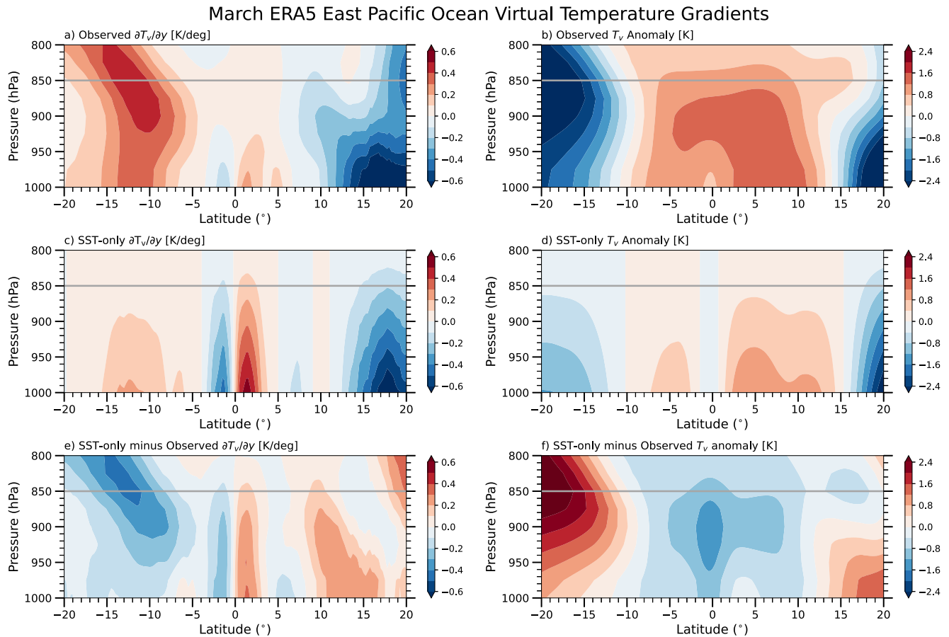
Figure 2. Same as Figure 1 but for March.
