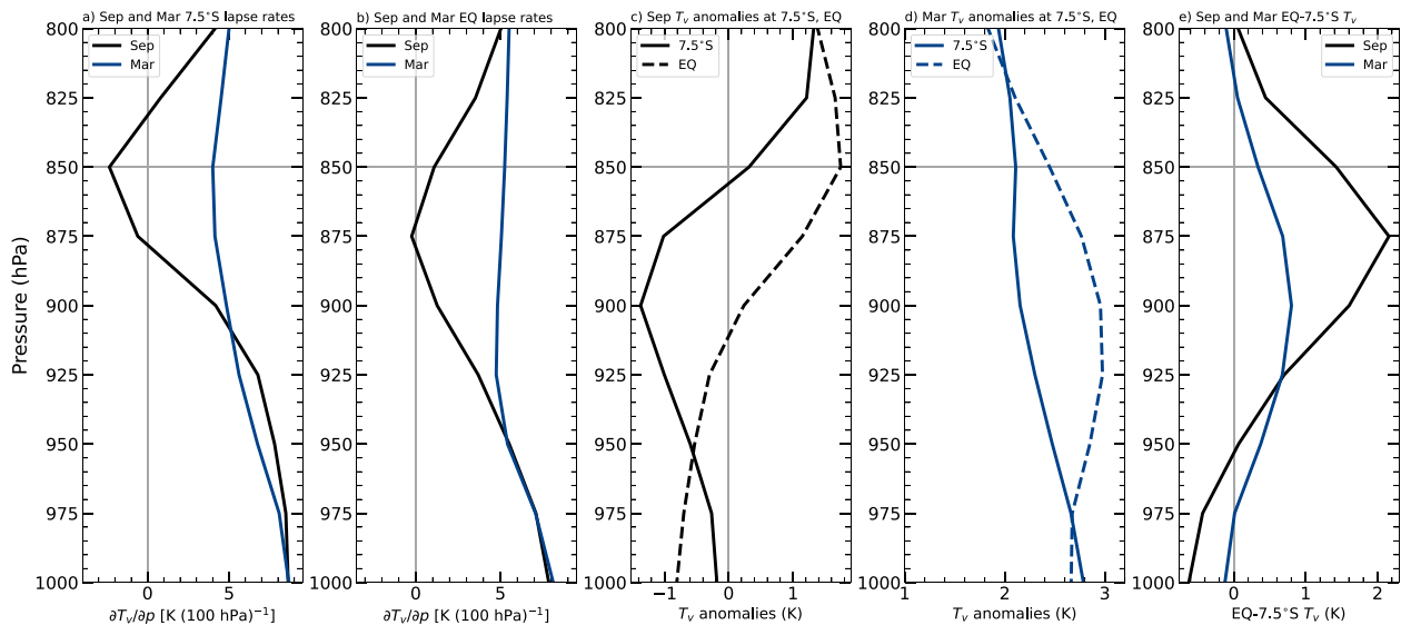
Figure 6. ERA5 \partial T_v / \partial p over the east Pacific Ocean (90–125°W) at (a) 7.5°S and (b) EQ for September (black) and March (blue). T_v anomaly (relative to the 30°S–30°N mean T_v ) at 7.5°S (solid) and EQ (dashed) for (c) September (black) and (d) March (blue). (e) EQ minus 7.5°S T_v for September (black) and March (blue), which highlights the change in direction of the T_v gradient near 950–975 hPa.
