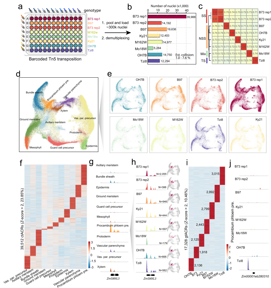
Fig. 2 Multiplexing eight samples with scifi-ATAC-seq. a Well assignment showing the multiplexing of primary samples and genotypes. b Number of profiled nuclei for each genotype. Est. Collision: estimated cell barcode collisions within the same genotype. c Spearman correlation heatmap among the 8 libraries (SS, stiff stalk; NSS, non-stiff stalk; TS, tropical/subtropical; Mix, mixed tropical-temperate). d UMAP of all nuclei ( n = 124,656 ). Nuclei are colored by their predicted cell type. Vas. par. precursor: vascular parenchyma precursor, procambium phloem pre.: procambium phloem precursor. e UMAP of all nuclei across the eight samples. f Chromatin accessibility of cell-type-specific accessible chromatin regions (ctACRs, Z\text{-score} > 2 ) among all cell types. g Pseudobulk cell type Tn5 integration site coverage around the phloem precursor marker ZmSMXL3 . h Pseudobulk cell type Tn5 integration site coverage and UMAP embeddings overlaid with gene chromatin accessibility around the ZmSMXL3 . N, nuclei number of procambium phloem precursor. i Chromatin accessibility of genotype-specific accessible chromatin regions (gtACRs) among seven genotypes. The number of gtACRs was labeled. j Pseudobulk cell type Tn5 integration site coverage with gene chromatin accessibility around the Zm00001eb280310 across all samples in procambium phloem precursor cells
