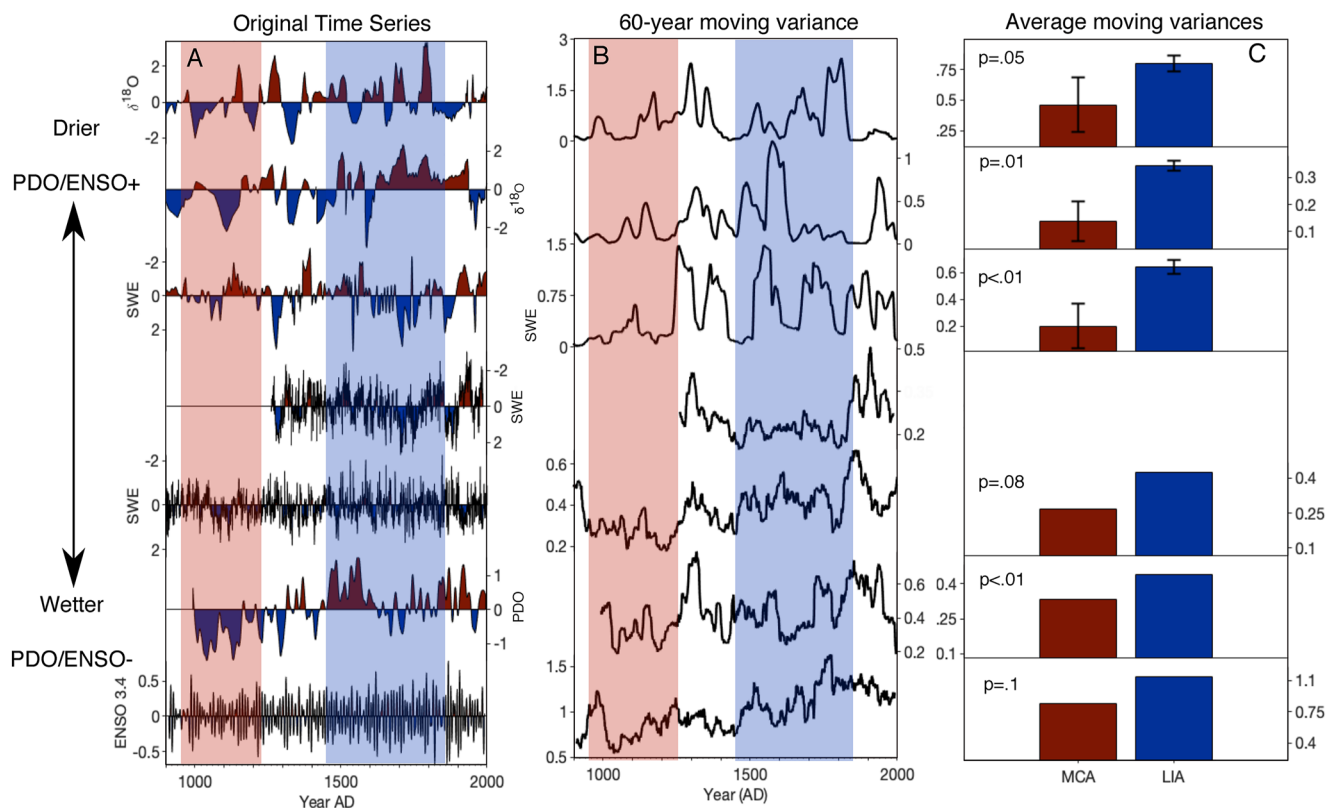
Figure 3. (a) Round and Castor lakes \delta^{18}\text{O} records (this study), Foy Lake, MT (Schoenemann et al., 2020), Upper Columbia River Basin and Southern Upper Colorado snow water equivalence reconstructions (Pederson et al., 2011), Western North America tree-ring based Pacific Decadal Oscillation reconstruction (MacDonald & Case, 2005), North American tree-ring El Niño Southern Oscillation reconstruction (Li et al., 2011) (all treated with 20-year smoothing). (b) 60-year moving variances of the same proxies. Red and blue shading indicates the Medieval Climate Anomaly (900–1250 CE) and Little Ice Age (1450–1850 CE), respectively. (c) Average 60-year moving variance for each proxy record. P -values indicate results of 2 sample Kolmogorov-Smirnov tests. Error bars on lake sediment records represent 97.5–2.5 percentile age model uncertainty (Castor and Round Lake) and proxy uncertainty (Foy Lake).
