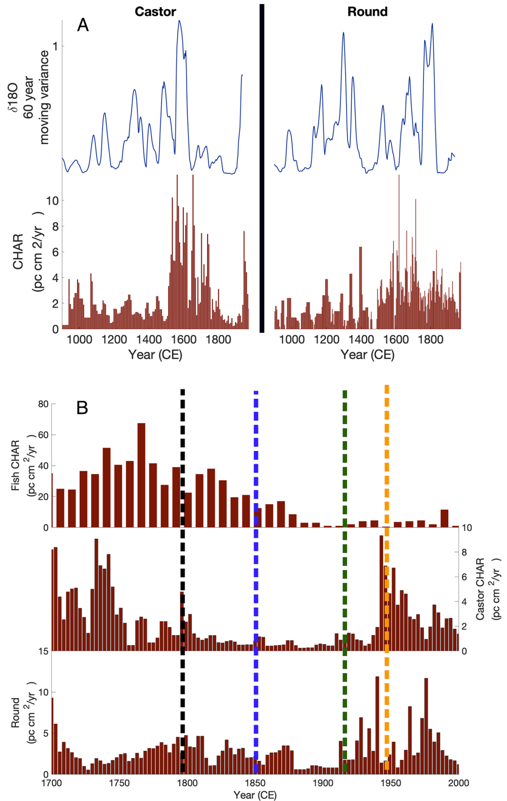
Figure 4. (a) Charcoal accumulation rate (CHAR) and 60-year moving average of variances of \delta^{18}\text{O} from Castor and Round lakes over the past millennium. (b) CHAR from Fish, Castor, and Round Lake between 1700 and 2000 CE. Black line indicates the first documented smallpox case (Boyd, 1999) among Native American groups in the region, blue line indicates the establishment of Euro-American grazing practices in the region (Walsh et al., 2018), green line represents onset fire suppression policies and orange line represents post-WWII increase in fire suppression efficacy.
