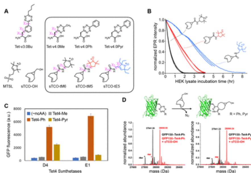
Figure 1. Tet-v4.0 ncAAs and sTCO-nitroxides: Spin-label Stability, Genetic Encoding, and Reactivity.
