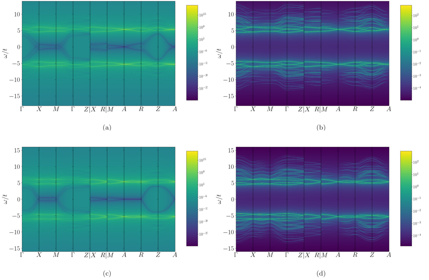
FIG. 13. Green's function determinant and spectral function for Hamiltonians invariant under space groups P4_2/mbc1' (No. 135) (top row) and P4/ncc1' (No. 130) (bottom row) with HK interactions H_{\text{HK}}^1 + H_{\text{HK}}^2 + H_{\text{HK}}^3 at half filling (four electrons per unit cell). In the left two panels [(a), (c)], we show the absolute value of the determinant |\det(G^+(\mathbf{k}, \omega))| , and in the right two panels [(b), (d)], the spectral function -\frac{1}{\pi} \text{Im Tr}(G^+(\mathbf{k}, \omega)) . The band of zeros in the determinant of the orbital model demonstrates that models in both space groups remain Mott insulators when the ground state becomes nondegenerate. (a) |\det(G^+(\mathbf{k}, \omega))| for the space group P4_2/mbc1' (No. 135) Hamiltonian H_{135}^0 + H_{\text{HK}}^1 + H_{\text{HK}}^2 + H_{\text{HK}}^3 . (b) Spectral function, -\frac{1}{\pi} \text{Im Tr}(G^+(\mathbf{k}, \omega)) , for H_{135}^0 + H_{\text{HK}}^1 + H_{\text{HK}}^2 + H_{\text{HK}}^3 . (c) |\det(G^+(\mathbf{k}, \omega))| for space group P4/ncc1' (No. 130) Hamiltonian H_{130}^0 + H_{\text{HK}}^1 + H_{\text{HK}}^2 + H_{\text{HK}}^3 . (d) Spectral function, -\frac{1}{\pi} \text{Im Tr}(G^+(\mathbf{k}, \omega)) , for space group P4/ncc1' (No. 130) Hamiltonian H_{130}^0 + H_{\text{HK}}^1 + H_{\text{HK}}^2 + H_{\text{HK}}^3 . The parameter values for space group P4_2/mbc1' (No. 135) are t_{xy} = 1 , t_z = 0.5 , t'_1 = 0.3 , t'_2 = 0.3 , \lambda'_1 = 0.5 , \lambda'_2 = 0.1 , \lambda'_3 = 0.15 , U_1 = 4 , U_2 = 2 , U_3 = 4\mu_0 = 4 . The parameter values for space group P4/ncc1' (No. 130) are t_{xy} = 1 , t_z = 0.5 , \lambda_1 = 0.3 , \lambda_2 = 0.3 , \lambda_3 = 0.3 , U_1 = 4 , U_2 = 2 , U_3 = 2 , \mu_0 = 4 .
