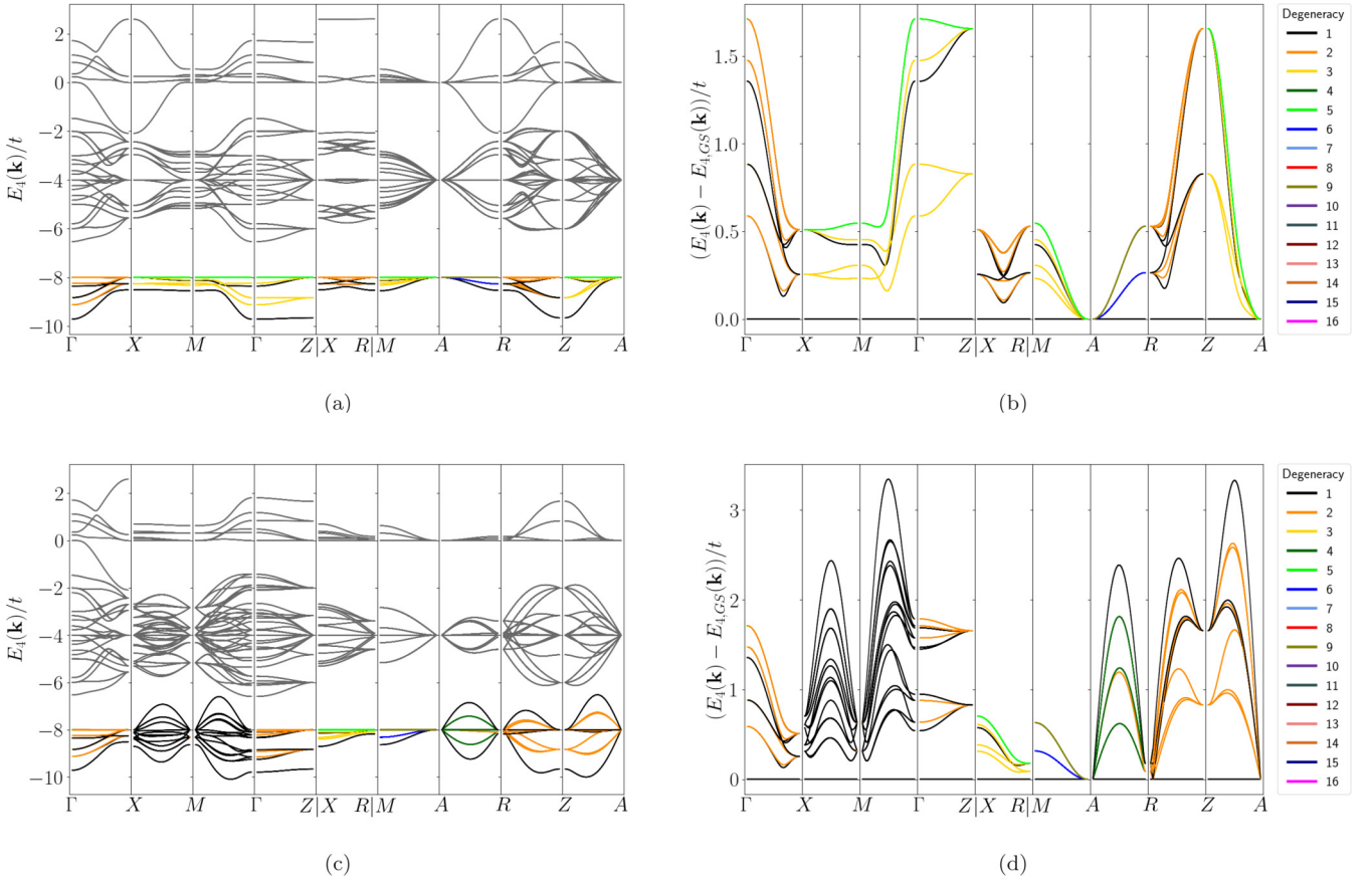
FIG. 9. Spectra along the high-symmetry paths (HSPs) for space group P4_2/mbc1' (No. 135) (top row) and space group P4/ncc1' (No. 130) (bottom row) with HK interactions H_{HK}^1 in the half-filled (four electrons per unit cell) sector. The low-energy states have been colored according to their degeneracy, given in the rightmost panel. The degeneracy of the higher energy states has been grayed out for clarity. (a) Spectrum E_4(\mathbf{k}) of the orbital HK model in space group P4_2/mbc1' (No. 135) with HK interaction H_{HK}^1 in the four-particle sector. (b) Low-energy part of the excitation spectrum E_4(\mathbf{k}) - E_{4,GS}(\mathbf{k}) . Here we show only the 16 states below the gap. (c) Spectrum E_4(\mathbf{k}) of the orbital HK model in space group P4/ncc1' (No. 130) with HK interactions H_{HK}^1 in the four-particle sector. (d) Low-energy part of the excitation spectrum E_4(\mathbf{k}) - E_{4,GS}(\mathbf{k}) for the model in space group P4/ncc1' (No. 130). Note that the ground state is nondegenerate at the A point and along the line R-Z . The parameter values for space group P4_2/mbc1' (No. 135) are t_{xy} = 1 , t_z = 0.5 , t'_1 = 0.3 , t'_2 = 0.3 , \lambda'_1 = 0.5 , \lambda'_2 = 0.1 , \lambda'_3 = 0.15 , U_1 = 4 , \mu_0 = 2 . The parameter values for space group P4/ncc1' (No. 130) are t_{xy} = 1 , t_z = 0.5 , \lambda_1 = 0.3 , \lambda_2 = 0.3 , \lambda_3 = 0.3 , U_1 = 4 , \mu_0 = 2 .
