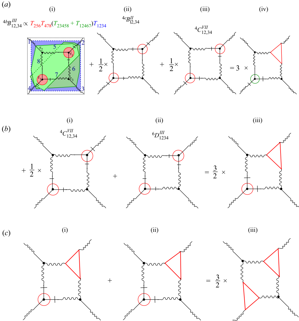
Figure 14. The last group of the square diagrams for 4F_{1234}^{(4)} , with two earliest time zones producing the product T_{256}T_{478} . As in figure 12(b-i), the relationship between \tau_2 and \tau_3 resulting in the sum of two contributions ( T_{23458} + T_{12467} ) originated from two overlapping green zones.
