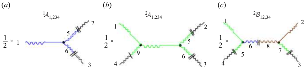
Figure 3. The lowest-order contributions to (a) the three-point correlator {}^3\mathcal{F}_{123}^{1A} and (b,c) the four-point correlator {}^3\mathcal{F}_{1234}^{2A} and {}^3\mathcal{F}_{1234}^{2B} as a result of gluing of three and four trees, separated by \parallel . All diagrams include prefactors. The operator \mathbf{P} is not shown explicitly on this and subsequent diagrams, but its presence is implied.
