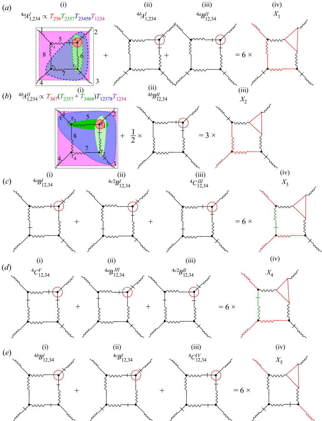
Figure 12. Five subgroups of the square diagrams for {}^4F_{1234}^{(4)} with cancellation in each line. Notation and colour codes of the time zones and interaction times are the same as in previous figures. The new element appears in (b-i): the relationship between \tau_2 and \tau_3 is not dictated by the orientation of the Green's functions. Consequently, integrations over \tau_2 and \tau_3 are performed differently in these two cases. If \tau_2 < \tau_3 , then the \tau_2 integration occurs over the region coloured in light green, while the \tau_2 > \tau_3 region is coloured in darker green. Such a partition of integration regions leads to the sum of two contributions ( T_{2357} + T_{3468} ) originated from these two green zones.
