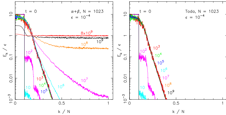
Fig. 1. Energy spectrum plotted as a function of k/N at selected times. Left: FPUT simulations; Right: Toda simulations. See text for details. Source: Plot taken from Ref. [124].
