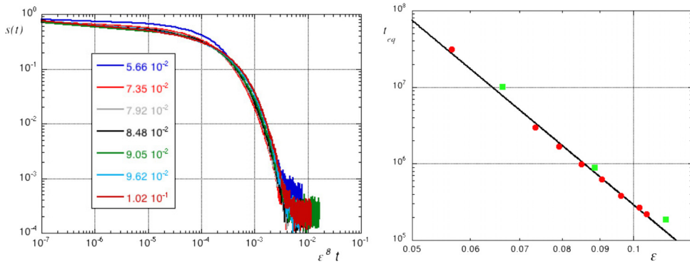
Fig. 2. Left: Entropy s(t) as a function of \epsilon^8 t for different simulations of the \alpha -FPUT system characterized by different values of \epsilon . Right: Equipartition time as a function of \epsilon in Log-Log coordinates. See [157] for details.
