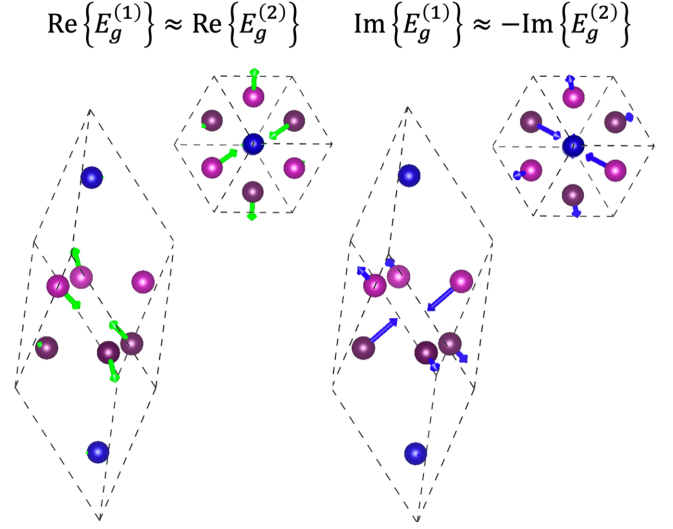
FIG. 2. Visualization of the real and imaginary components of the chiral phonons E_g^{\delta 1p} and E_g^{\delta 2p} . Cr atoms are depicted in blue, while top-layer and bottom-layer I atoms are in bright and dark magenta, respectively. The green vectors represent the real part of the phonon displacement, and the blue vectors represent the imaginary part. The real part of E_g^{\delta 1p} and E_g^{\delta 2p} are nearly identical, while the imaginary parts are in opposite directions.
