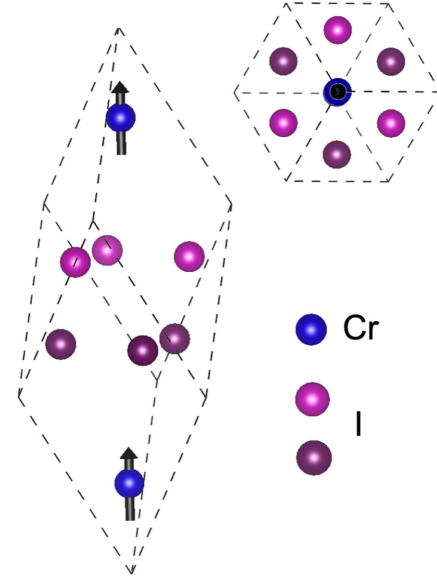
FIG. 1. Visualization of crystal structure and magnetic moments of a bulk \text{CrI}_3 unit cell. Cr atoms are depicted in blue, while top-layer and bottom-layer I atoms are in bright and dark magenta, respectively. The black vectors indicate the magnetic moments, which are oriented along the z direction.
