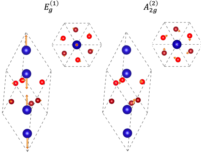
FIG. 5. ARPAM for two selected modes in bulk \text{Cr}_2\text{O}_3 : E_g^{\delta_{1p}} -like mode near 36 meV and A_{2g}^{\delta_{2p}} -like mode near 57 meV. The ARPAM for the E_g -like mode is traced over two degenerate modes. The amplitude of ARPAM in this figure is amplified by a factor of 1000 compared to Fig. 6.
