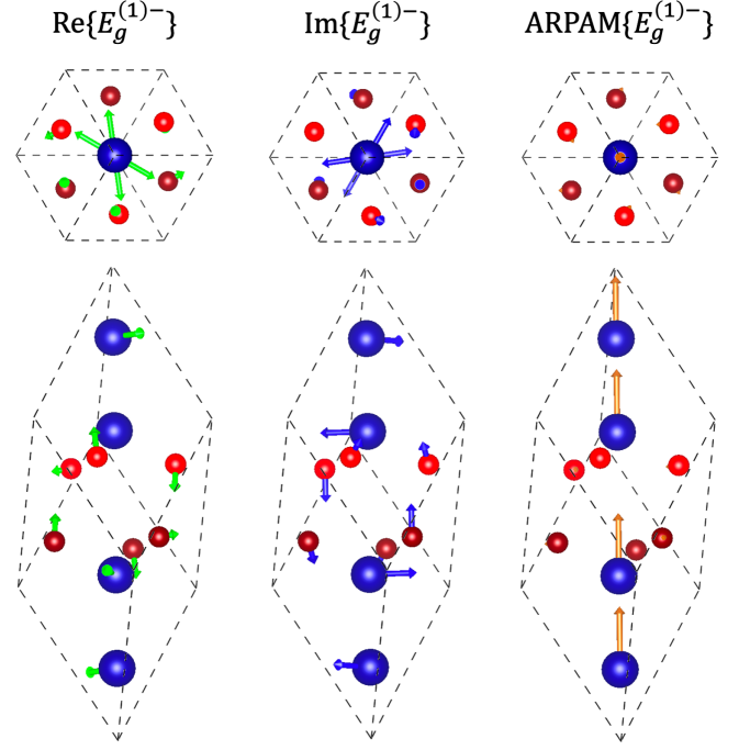
FIG. 6. The real and imaginary components, as well as ARPAM, of the chiral phonon E_g^{\delta_{1p-}} around 36 meV in \text{Cr}_2\text{O}_3 . The Cr atoms are shown in blue, while the top-layer and bottom-layer O atoms are depicted in bright and dark red, respectively. The green vectors indicate the real part of the phonon displacement, the blue vectors indicate the imaginary part, and the brown vectors represent the ARPAM. The real parts of E_g^{\delta_{1p}} are almost identical to E_g^{\delta_{1p-}} , while its imaginary parts and ARPAM are almost opposite to those of E_g^{\delta_{1p-}} .
