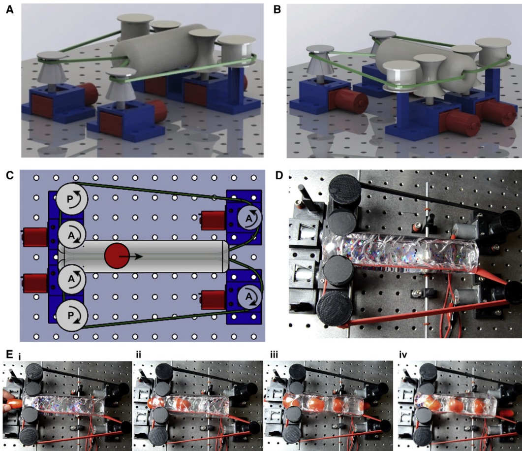
Figure 4. Conveying with a toroidal hydrostat
