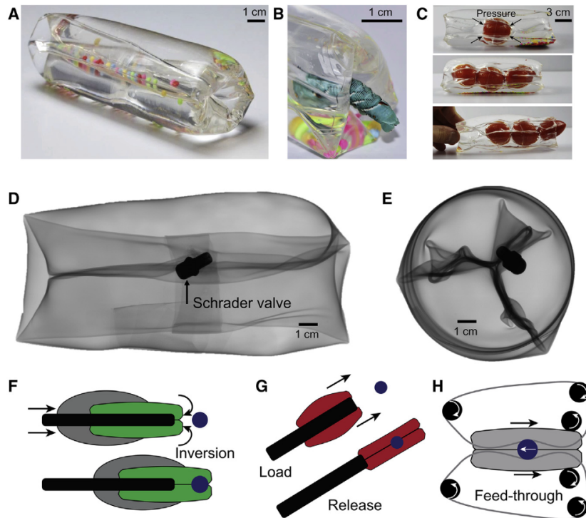
Figure 1. A soft, toroidal hydrostat
