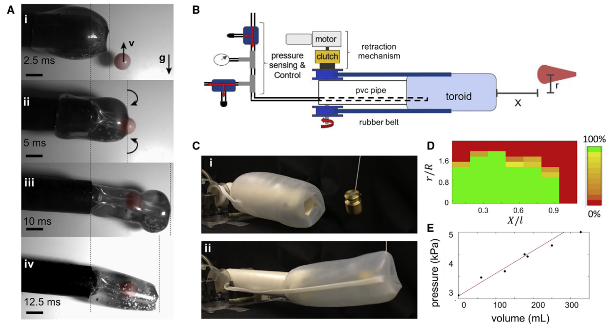
Figure 3. Catching with a catapulting toroidal hydrostat
