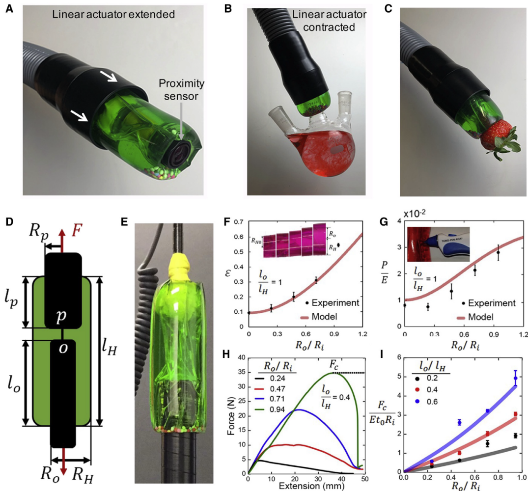
Figure 2. Gripping with a toroidal hydrostat
