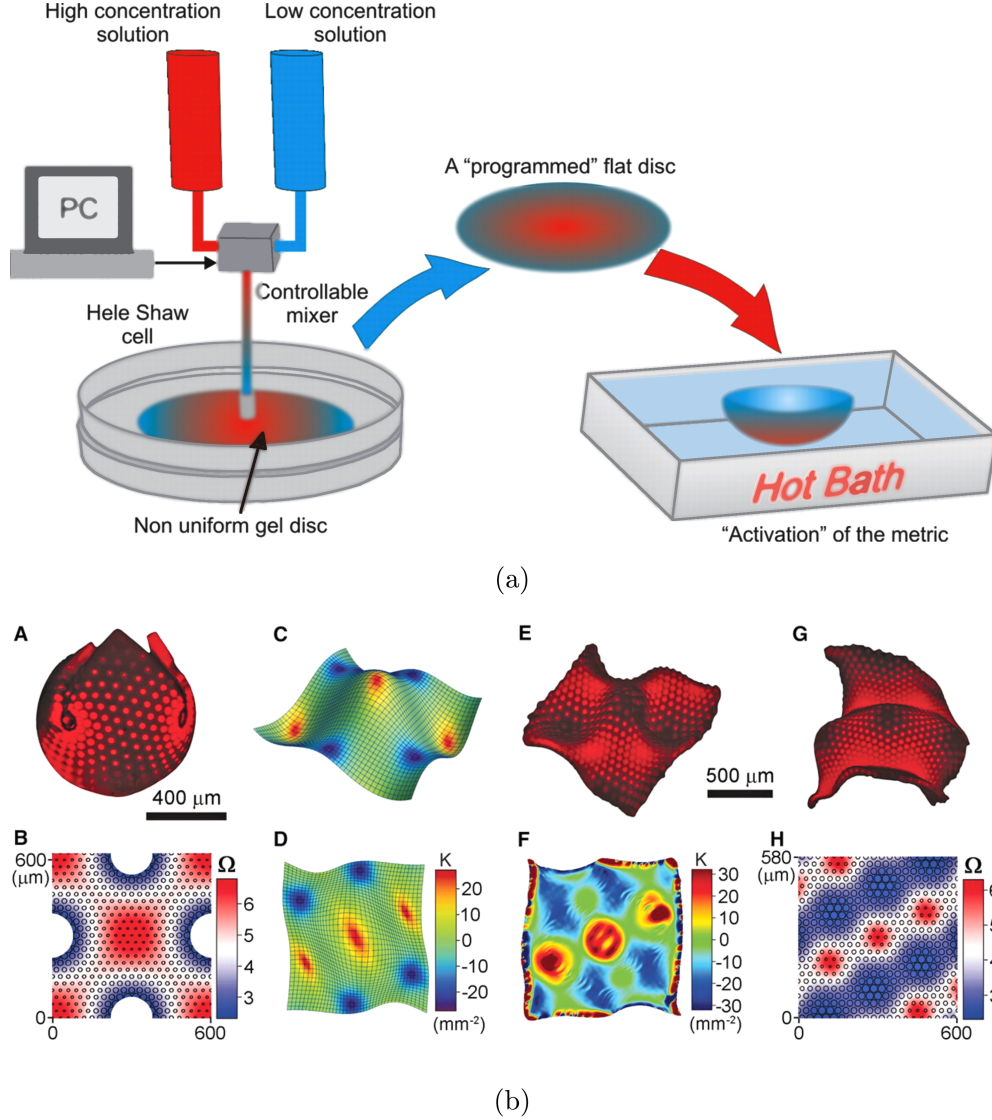
FIGURE 4. Imposing nontrivial target metrics in sheets of NIPA gels. The figures shown are (a) radially symmetric discs cast by injecting the solution into the gap between two flat glass plates through a central hole [64, © 2007, reprinted with permission from AAAS], (b) nonaxisymmetric swelling patterns constructed by half-tone gel lithography in [63, © 2012, reprinted with permission from AAAS].
