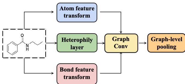
Figure 2: Graph Encoder, including atom and bond feature propagation, as well as graph-level pooling.
