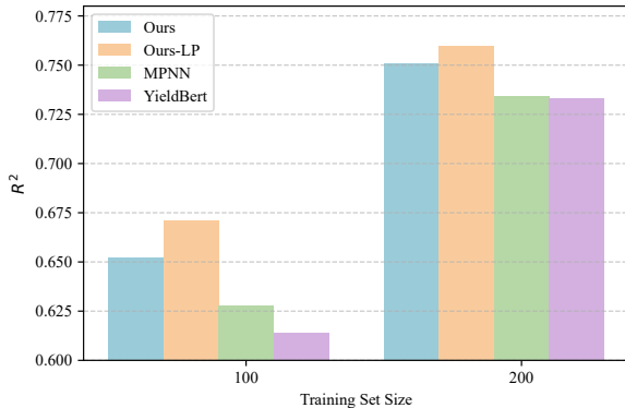
Figure 3: Label efficient learning performance on the Buchwald–Hartwig reactions dataset.
