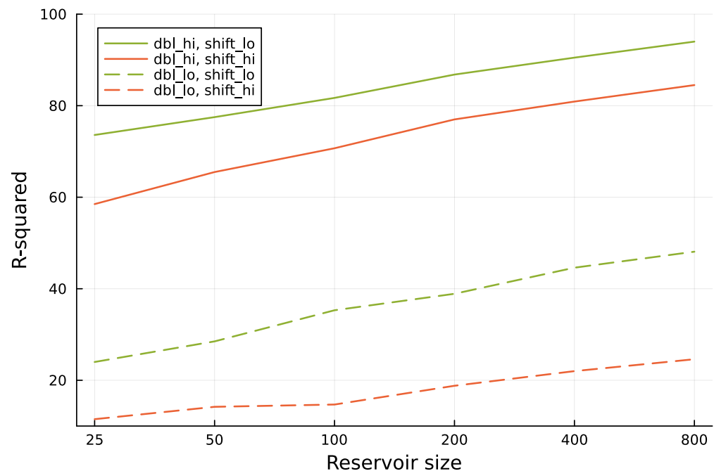
Figure 4. Increasing reservoir size provides better predictions for future environmental state. The analysis follows the methods used in Figure 3. Here, dbi_lo denotes a doubling time of approximately 0.52, and dbi_hi denotes a doubling time of approximately 1.42. The value of shift_lo denotes a prediction into the future over 1.0 time units, and shift_hi denotes a prediction into the future over 2.0 time units. The six different reservoir sizes used in the computer runs are shown as labels for the tick marks along the x-axis.
