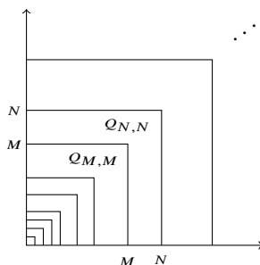
Figure 1. Family of nested rectangles (cubes) Q_{M,M} \subset Q_{N,N} with M < N , for k = 2 .
