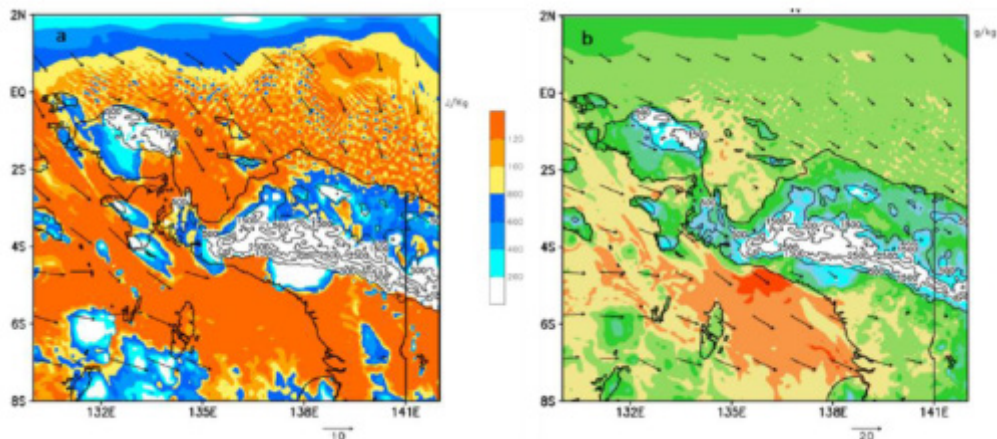
Figure 15. (a) CAPE from the surface to 850 hPa (b) water vapor mixing ratio ( q_v )
