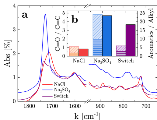
Figure 4. Adsorption reversibility. The switch film ( \text{NaCl} \Rightarrow \text{Na}_2\text{SO}_4 ) is compared to the ones formed independently with NaCl and \text{Na}_2\text{SO}_4 salt (all of 0.1 M concentration), showing the acid region of the FTIR spectra (1500–1900 \text{cm}^{-1} ) and the fingerprint region (650–950 \text{cm}^{-1} ). (b) Quantification of relative concentrations of carboxylic acids (dashed diagonal: bound; dashed horizontal: free) and aromatics (solid bars) using the areas of deconvoluted peaks. The salt switch film appears to be a combination of individual salt films.
