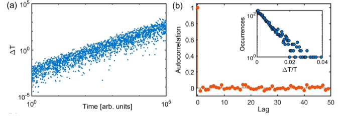
FIG. 2. Stochastic simulation of the crackling statistics assuming a broad relaxation rate distribution (3000 modes with rates between 10^{-6} and 10). (a) The typical time gaps between consecutive events increase linearly with time, as predicted theoretically. (b) Since the model assumes transitions between independent two-level systems, the autocorrelation of time gaps vanishes for nonzero lags. Inset: upon rescaling time, the time gap distribution becomes exponential, as shown analytically in the main text.
