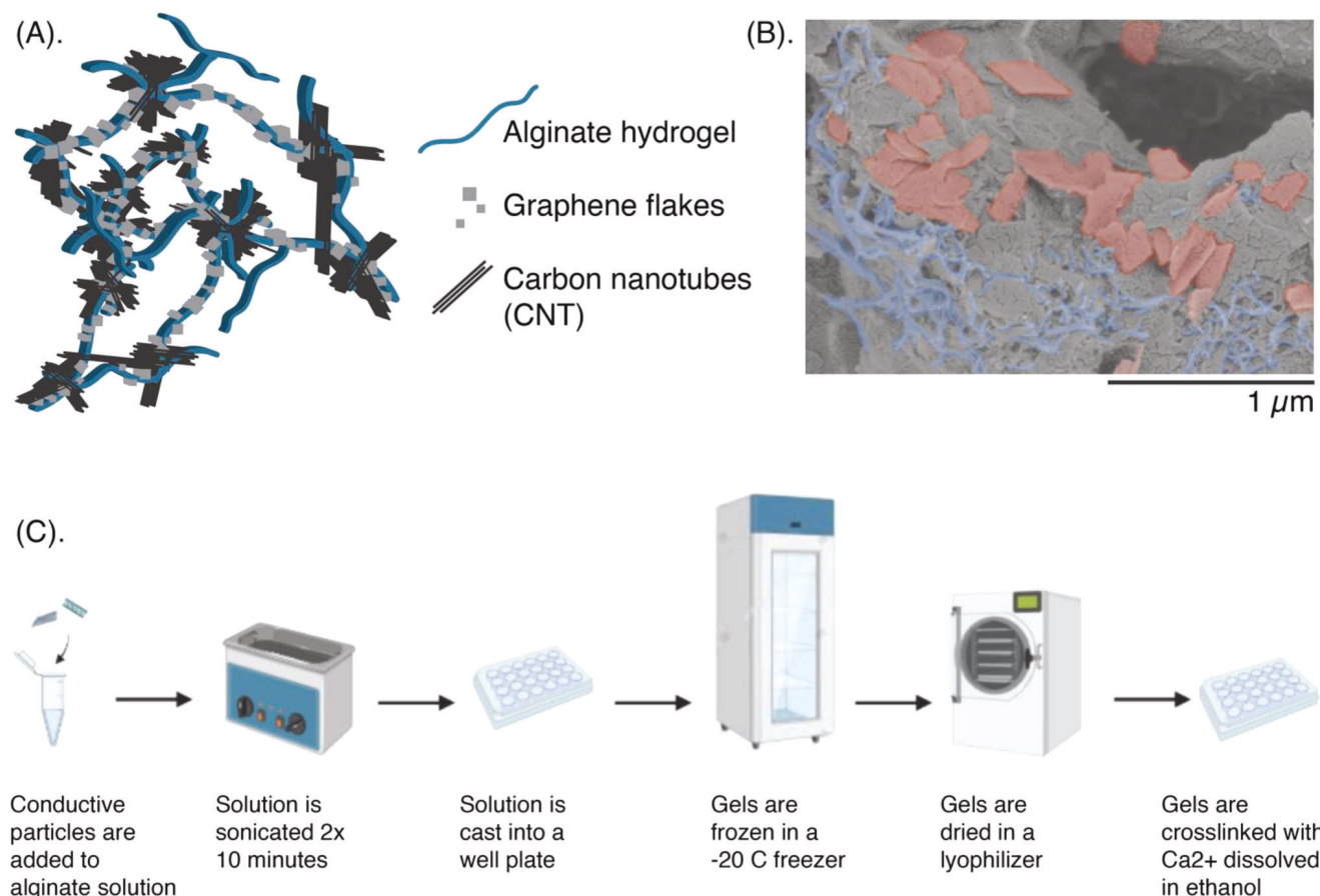
Figure 1. A porous biomaterial scaffold with embedded carbon nanomaterials. A) Schematic of the scaffold, with a porous matrix of alginate (blue) that mechanically traps conductive carbon nanomaterials such as graphene flakes (GF, gray squares) and/or carbon nanotubes (CNT, black lines). B) Scanning electron microscopy (SEM) micrographs of the scaffold, with the alginate left gray, the GFs falsely colored in red, and the CNTs falsely-colored in blue. Scale bar: 1 \mu\text{m} . C) Schematic showing the fabrication of the porous scaffolds.
