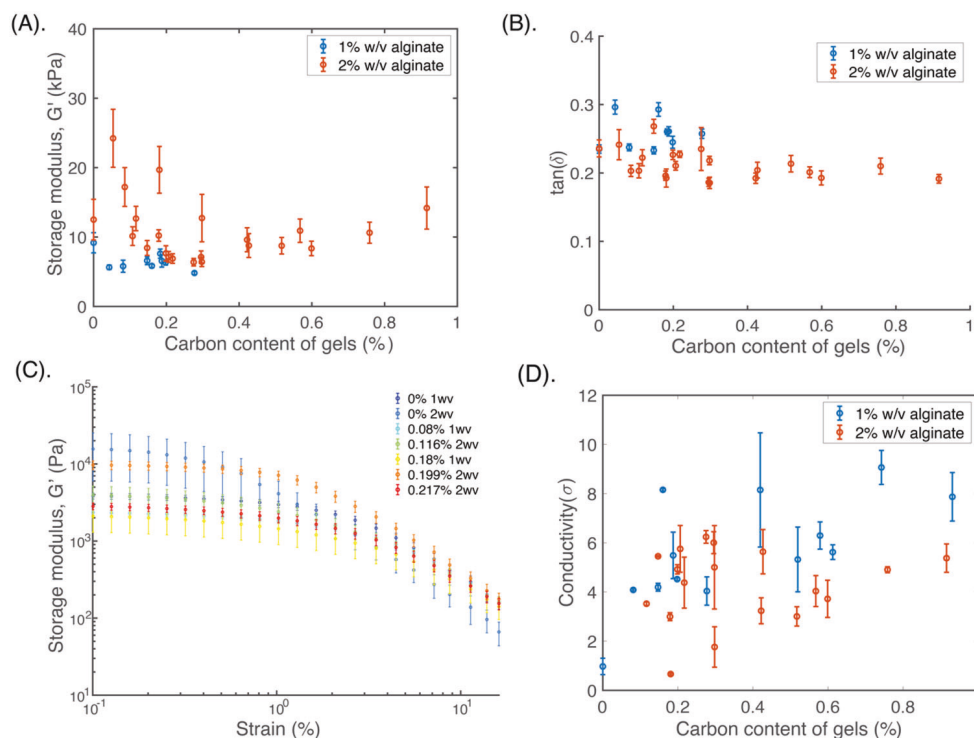
Figure 2. Electrical properties of the scaffold can be adjusted by varying amounts of each carbon nanomaterial, while keeping mechanical properties largely consistent. A) Quantification of the storage modulus ( G' ), and B) \tan(\delta) of the scaffolds with varying amounts of total carbon (graphene flakes and carbon nanotubes) using nanoindentation analysis ( N = 6 independent gels, n > 5 measurements per gel). Gels with 1% (blue) and 2% (red) w/v alginate content are compared. Mean and standard error are shown for each graph. C) Quantification of the bulk G' versus % strain, with varying amounts of carbon (%) and with either 1% or 2% w/v alginate. N = 4 independent gels for each composition. Legend (right) denotes the alginate w/v % of the composite, and the total amount of additive in the scaffold (%). D) Quantification of gel conductivity with varying amounts of carbon, for 1% (blue) and 2% (red) w/v alginate. N = 5 independent gels for each composition, with n > 12 measurements per gel. Mean and s.d. are shown for each graph.
