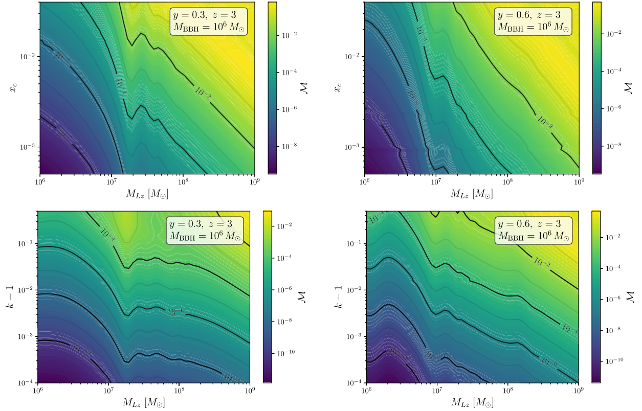
FIG. 11. Mismatch between CIS and SIS (top row), and gSIS and SIS (bottom row) for impact parameter y = 0.3 (left column) and y = 0.6 (right column) for a source mass M_{\text{BBH}} = 10^6 M_\odot . The mismatch is evaluated for different lens masses M_{Lz} and by varying the lens parameter of the lens ( x_c for CIS and k for gSIS).
