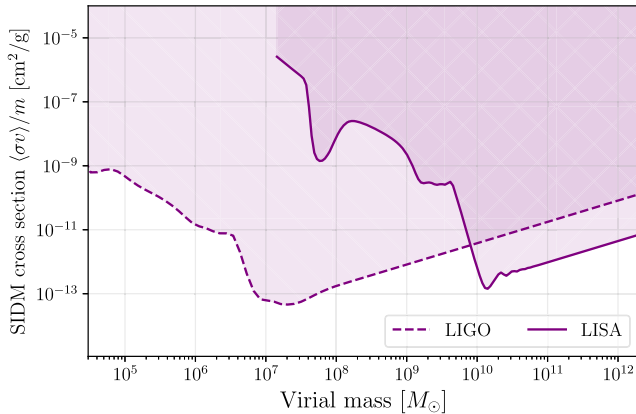
FIG. 22. GW lensing as a probe of SIDM for the CIS profile. The shaded regions can be probed by strongly lensed GWs. Here y = 0.6 , z_S = 3 , M_{\text{BBH}} = 10^6 M_{\odot} , \text{SNR} = 10^3 for LISA and z_S = 0.2 , M_{\text{BBH}} = 30 M_{\odot} , \text{SNR} = 10^2 for LIGO. The lens redshift is chosen to minimize the projected core size (see text). Constraints on the cross section scale as \propto \rho(r_c) , Eq. (71). Therefore, results for an NFW profile are expected to scale as the square root of the CIS ones, compare Eqs. (72) and (73). The forecasted CIS results are orders of magnitude tighter than existing constraints [70]. Ultimately, probes based on very small cores (low \langle\sigma v\rangle/m ) will be limited by astrophysical uncertainties.
