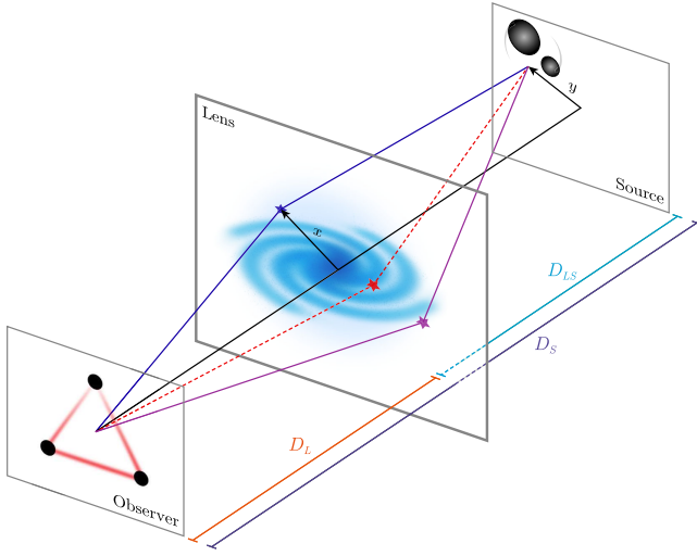
FIG. 1. Setup for strong gravitational lensing. A lens located at (angular diameter) distance D_L magnifies a source at D_S with (dimensionless) impact parameter \mathbf{y} . In the geometric-optics limit, the lens produces multiple images (stars), whose positions are given by the dimensionless coordinates \mathbf{x}_i in the lens plane. GWs allow us to observe all images, including the central image (red), whose EM counterpart is further suppressed ( 1 > \sqrt{|\mu|} > |\mu| ), and blocked or outshined by the lens matter.
