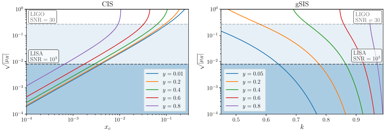
FIG. 10. Detectability criterion in GO: magnification of the third image as a function of the lens parameter. Magnifications above the threshold values \text{SNR}_{\text{th}} = 8 are detectable by GW experiments. Horizontal lines correspond to typical LIGO and LISA events, with SNR of 30 and 10^3 respectively. Left: CIS case, as a function of the core size x_c . Right: gSIS case, as a function of the slope parameter k .
