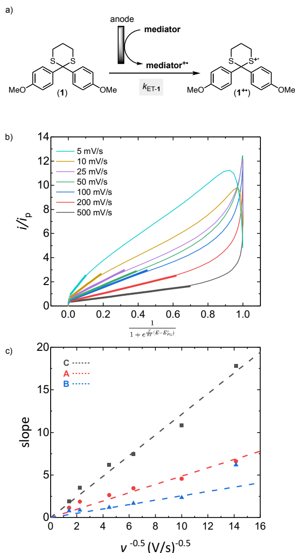
Figure 2. (a) Electron transfer between the oxidized mediator (mediator ++ ) and substrate 1 . (b) Foot of the wave analysis for mediator C . (c) Fitting to obtain k_{ET-1} for A-C .
