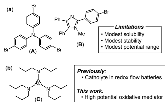
Figure 1. (a) Known high-potential oxidative mediators for electro-organic synthesis. (b) This work : Tris(amino)cyclopropeniums as mediators for electro-organic synthesis.
