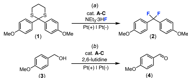
Scheme 1. Electrochemical oxidation reactions used to benchmark mediators A-C
