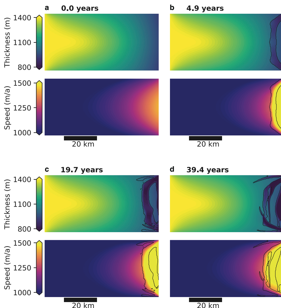
Figure 4. Evolution of rifts in an idealized ice shelf. Panel a shows a snapshot of the steady state ice thickness and speed at the beginning of the simulation. Panels b–d show snapshots at different points in time. Contours show fully failed regions. Supplementary animation M1 shows an animation over several centuries illustrating the sporadic detachment of bergs.
