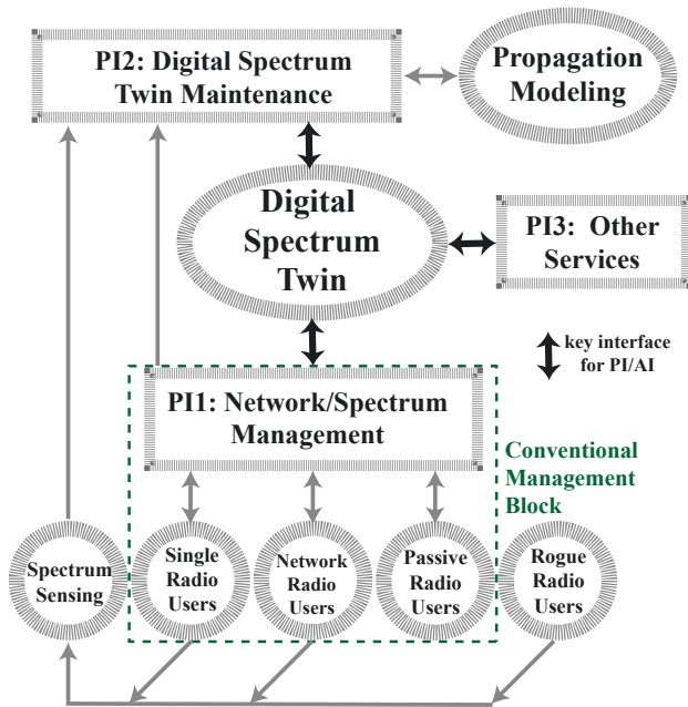
Fig. 1: Block diagram of a digital spectrum twin (DST) and its interfaces with other radios and operations in spectrum management.
