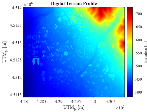
Fig. 11: Digital terrain profile showing a combination of the digital elevation map and the building layout in UTM zone 12. Map dimensions are approximately 2.6 km by 2.9 km with a 0.5 m resolution.
