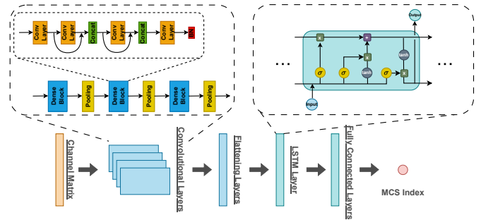
Fig. 2: ML-based framework.
