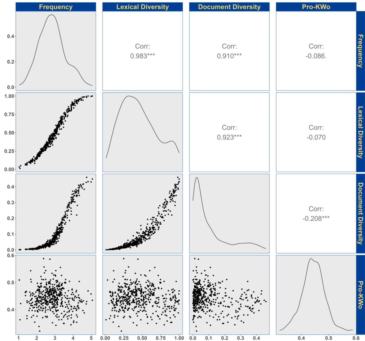
Fig. 1. Correlogram of all distributional statistics at 24 months. Frequency is the log 10 transformed cumulative frequency. The symbols *, **, and *** in the correlogram indicate the level of statistical significance of the correlation coefficients (p-values less than 0.05, 0.01, and 0.001 respectively).
