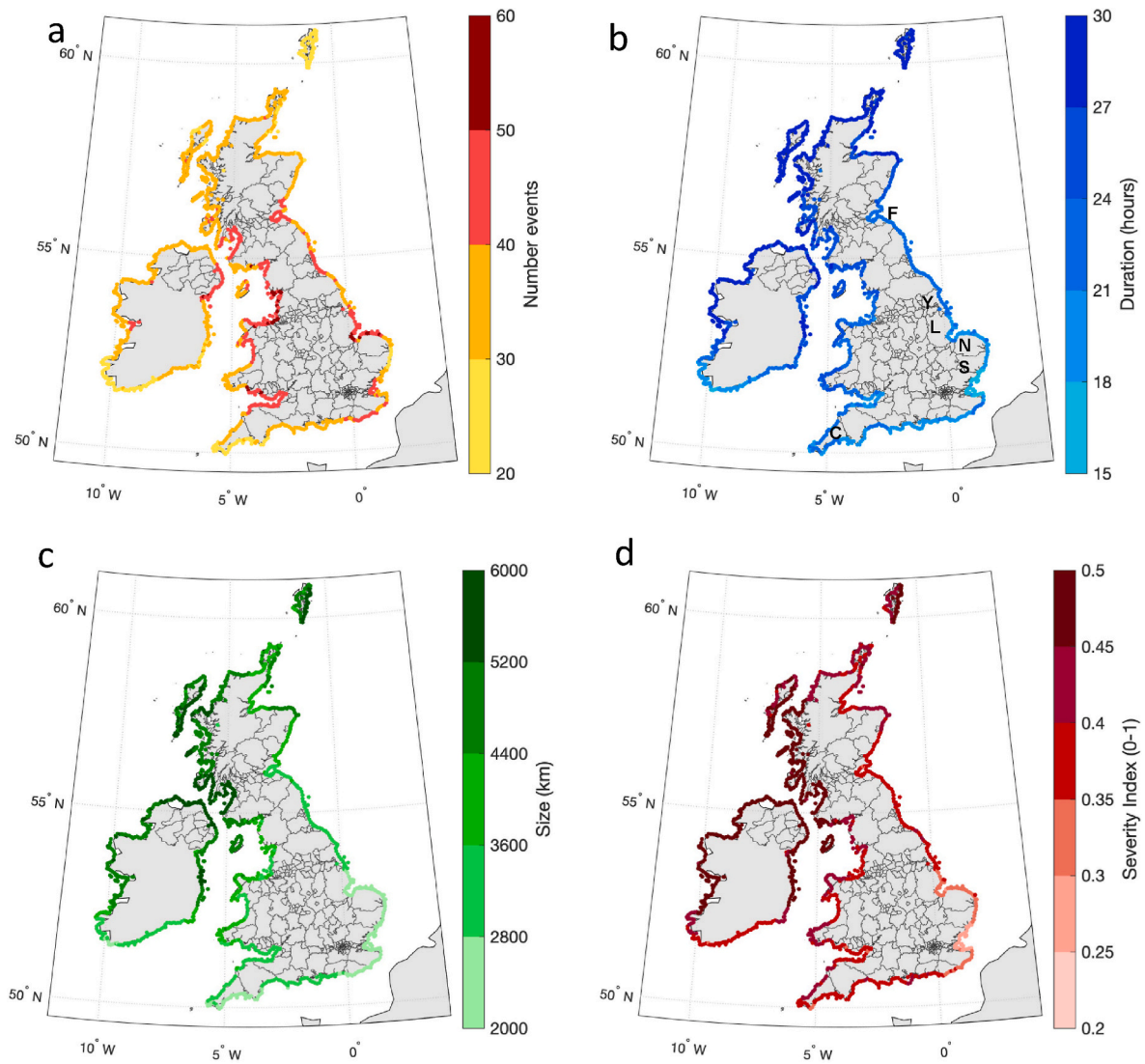
Fig. 6. Spatial characterization of the collection of 270 surge events: (a) number of events; (b) mean duration (in hours), (c) mean TH2 footprint size (in km of coastline where the surge level exceeded the TH2 threshold) and (d) mean value of the severity index (range value between 0 and 1) of all events that pass through each coastal site.
