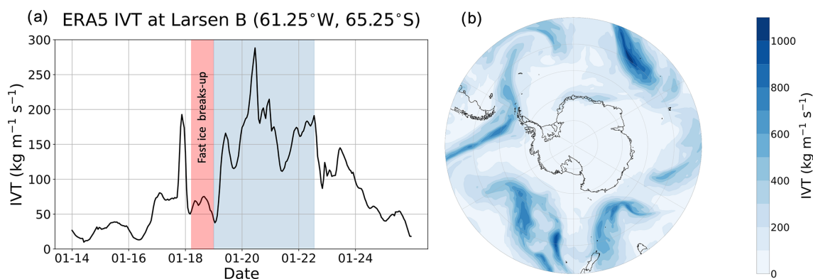
Figure 4. (a) Time series of IVT for January 2022 at 65.25° S, 61.25° W. (b) Map of ERA-5 IVT in the Southern Hemisphere at 11:00 UTC on 20 January 2022, during the peak IVT at Larsen B. The AR is identified as a long filament of high IVT that extends from the eastern Pacific across the Antarctic Peninsula and into the Atlantic Ocean. Red shading indicates the arrival of the swell and fast-ice breakup. Blue shading indicates the duration of the AR event over Larsen B.
