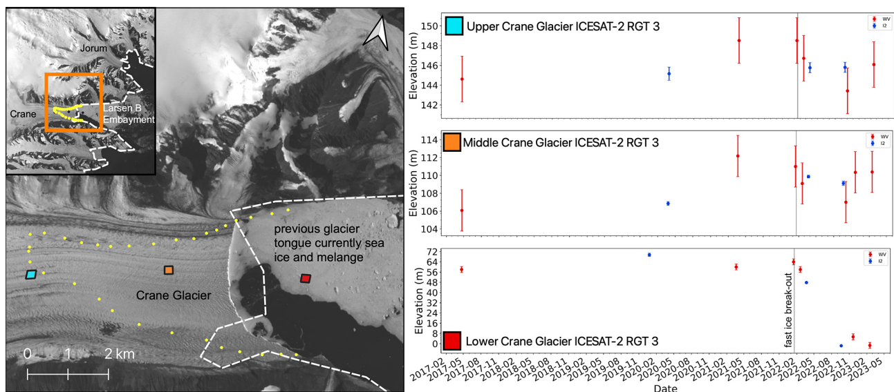
Figure 10. Crane Glacier near-centerline elevation changes through time. The background image is from Landsat 9, 17 January 2023. The time series plot corresponds to the area of the box of the same color. The gray band indicates the date of the fast-ice breakout event. Note the different vertical scales of the figure.
