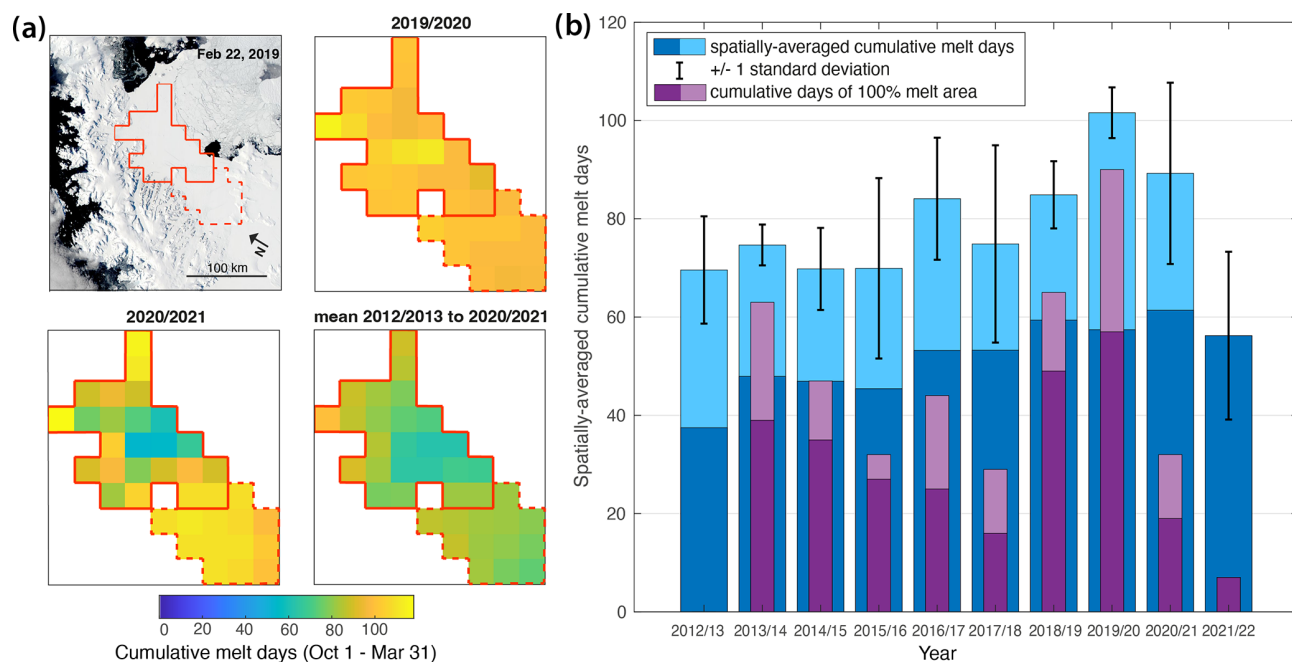
Figure 5. Cumulative melt days derived from AMSR-E/2 passive microwave melt data. (a) Cumulative melt days over the fast-ice area in the Larsen B embayment (area within solid red lines) and over the Scar Inlet Ice Shelf (area within dashed red line) for the 2019/2020 and 2020/2021 melt seasons, and the mean from 2012/2013 to 2020/2021. (b) Spatially averaged melt days (blue shades) and cumulative days of 100 % melt area (purple shades) over just the Larsen B embayment fast ice (solid red lines in panel a) from 2012/2013 to 2021/2022. The dark purple and dark blue bars show cumulative melt days from 1 October through 18 January (i.e., the data available for the 2021/2022 season), and the light purple and light blue bars show cumulative melt days from 1 October through 31 March.
