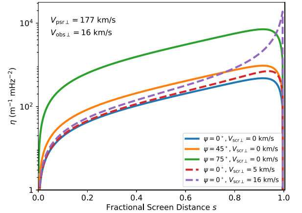
Figure 8. Arc curvature \eta versus screen distance s for different values of the screen velocity V_{\text{scr},\perp} and angle of anisotropy \psi , assuming V_{\text{psr},\perp} = 177 \text{ km s}^{-1} and V_{\text{obs},\perp} = 16 \text{ km s}^{-1} (as for B1929+10). Larger \psi and V_{\text{scr},\perp} both increase the possible values of \eta for a given s , and V_{\text{scr},\perp} has the largest effect on \eta near s \approx 1 when it is comparable to or greater than the observer velocity term.
