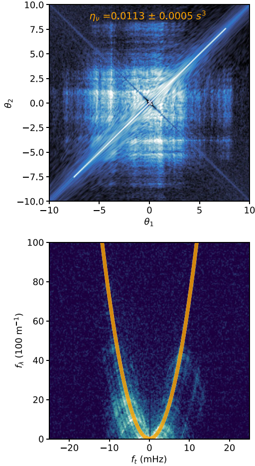
Figure A1. Top: The \theta – \theta diagram for J1740+1000 evaluated for the best fit curvature \eta_v = 0.0113 \pm 0.0005 \text{ s}^3 at 1375 MHz, equivalent to \eta = 72 \pm 5 \text{ m}^{-1} \text{ mHz}^{-2} . The main arc and reverse arclets are transformed into linear features that are parallel to the \theta – \theta axes, as expected (Sprenger et al. 2021; Baker et al. 2022). Here \theta_1 and \theta_2 are scaled sky coordinates in units of fringe frequency f_t , and could in principle be transformed into angular sky coordinates given knowledge of the effective velocity V_\perp (Baker et al. 2022). Bottom: The secondary spectrum measured in the 1.4 GHz frequency band. The best fit curvature inferred from the \theta – \theta transform is shown as the orange curve, the width of which is equal to the measurement uncertainty.
