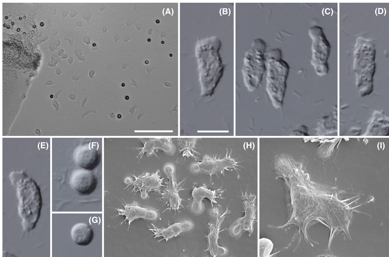
FIGURE 1 Light and scanning electron micrographs of Kanabo kenzan sp. nov., strain Union 16-1-3. (A) Diversity of trophic forms and cysts on the surface of an agar plate, scale bar = 100 \mu m; (B and C) Trophic cells, showing tubular form, subpseudopodia, and anterior locomotive hyaloplasm, scale bar = 10 \mu m (B–G to scale); (D) Trophic cell with nucleus and nucleolus visible in center of cell; (E) Trophic cell with distinct uroid and trailing finely tapered subpseudopodia; (F and G) Encysted amoebae; (H) SEM image of many trophic amoebae with distinct finely tapered subpseudopods and uroids, 3000X magnification, scale bar = 10 \mu m; (I) SEM image of single trophic amoeba, 7500X magnification, scale bar = 5 \mu m.
