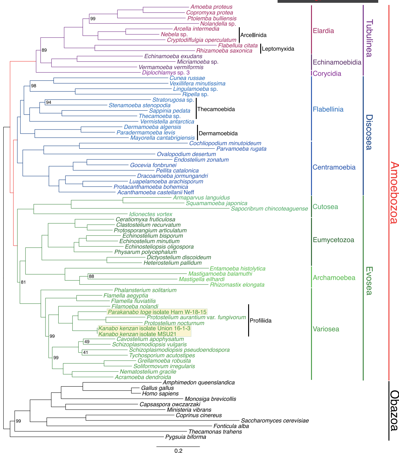
FIGURE 7 Maximum likelihood tree of Amoebozoa, using Obazoa as an outgroup, built with IQTree2 under LG+G4+F+C60+PSMF model. Constructed from a multigene concatenated matrix of 230 genes covering 73,839 total sites generated by PhyloFisher. Relevant clades are defined by labeled vertical bars, and our isolates are highlighted in yellow. The numbers at each node represent bootstrap values generated under the LG+G4+F+C60+PSMF model, and blank nodes represent full bootstrap support.
