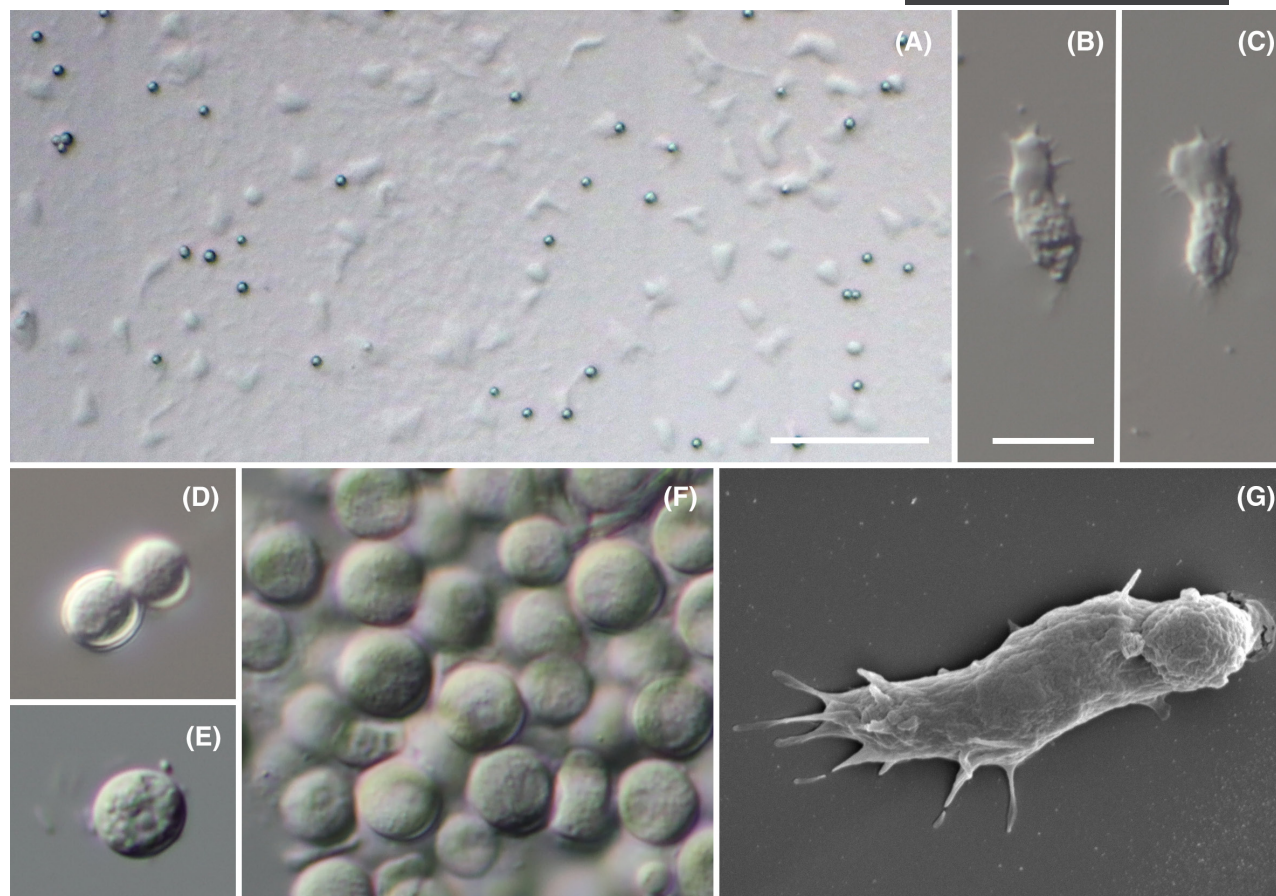
FIGURE 2 Light and scanning electron micrographs of Kanabo kenzan sp. nov., strain MSU2-1. (A) Diversity of trophic forms and cysts on the surface of an agar plate, scale bar=100 \mu m; (B and C) Trophic cells, showing tubular form, finely tapered subpseudopodia, anterior locomotive hyaloplasm, and nucleus and nucleolus, scale bar=10 \mu m (B–F to scale); (D and E) Cysts with nucleus visible; (F) Cluster of cysts; (G) SEM image of a single trophic amoeba, 10,000X magnification, scale bar=3 \mu m.
