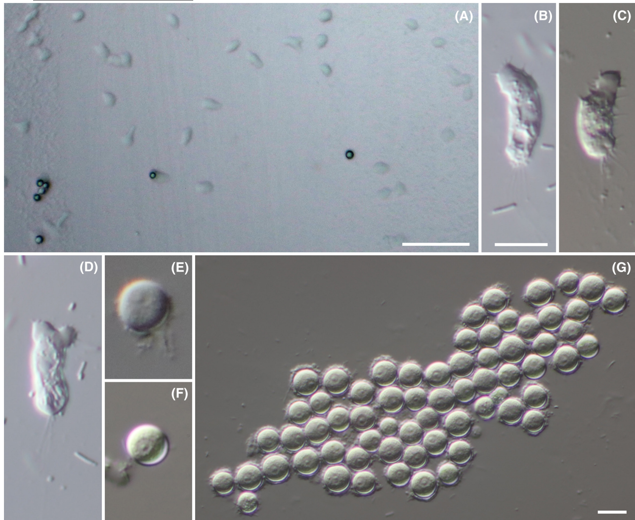
FIGURE 3 Light micrographs of Parakanabo toge sp. nov., strain Harn W-18-15. (A) Diversity of trophic forms and cysts on the surface of an agar plate scale bar=100 μm; (B and C) Trophic cells, showing tubular form, finely tapered subpseudopodia, anterior locomotive hyaloplasm, and trailing filopodia, scale bar=10 μm (B–F to scale); (D) Trophic cell with nucleus visible at its center; (E and F) Cysts with nucleus and nucleolus visible; (G) Cluster of cysts, scale bar=10 μm.
