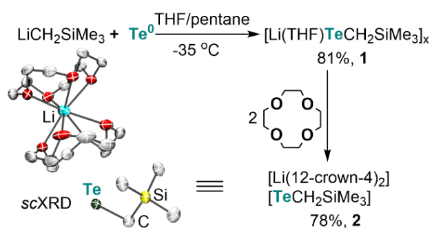
Scheme 1. Synthesis of tellurolate salts and the solid-state structure of the discrete tellurolate [Li(12-crown-4) 2 ][TeCH 2 SiMe 3 ] ( 2 ) with thermal ellipsoids at the 50% probability level and with H-atoms omitted for clarity.
