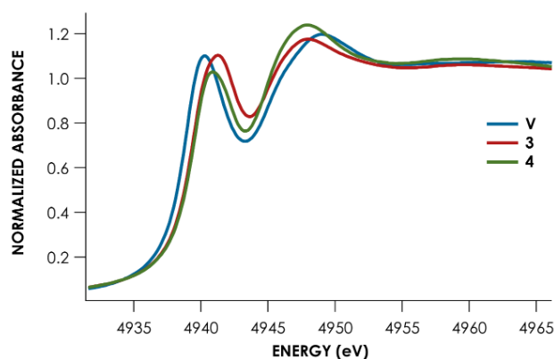
Figure 4. Te-L 1 edge XANES data for complexes V (blue), 3 (red), and 4 (green).
