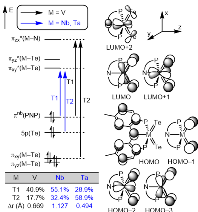
Figure 3. Conceptual MO diagrams of (PNP)M(Te) 2 (M = V, Nb, and Ta) complexes and the most contributing orbital transitions denoted as T1 and T2, respectively.
