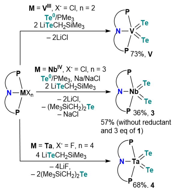
Scheme 2. Synthesis of the bis(tellurides) with the respective metal halide precursor to form complexes (PNP)M(Te) 2 (M = V; Nb, 3 ; Ta, 4 ). The PNP ligand is shown with a simplified cartoon omitting i Pr and aryl backbone groups.
