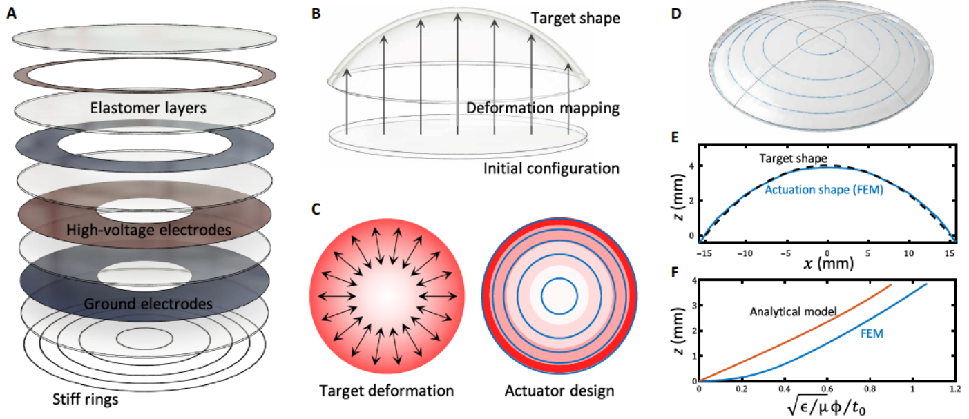
Figure 1. (A) Schematic exploded view of the structure of the shape-morphing DEA, designed to morph into a hemispherical cap, consisting of a multilayer of elastomers, separated by interdigitated ground and high-voltage electrodes, and a set of stiff rings that are 3D-printed onto the multilayer. (B) The initially flat elastomer sheet morphs into a hemispherical shape through a deformation mapping with zero lateral displacements and predefined out-of-plane displacement. (C) The deformation mapping (left) for morphing into the spherical cap consists of uniaxial actuations that are locally uniaxial along the radial direction, and their magnitude increases from zero at the center of the elastomer disk to the maximum at the edge. This target deformation is approximated by a set of stiff rings and active layers (right). Actuations along the rings are prevented, producing locally uniaxial deformations normal to the rings, and then the number of active layers determines the local magnitude of actuation. (D) The actuation shape for the actuator design in (A), simulated using finite element method (FEM), resembles the hemispherical target shape. (E) Quantitative comparison between the finite elements simulation of the actuation profile and the target shape. (F) Finite elements simulation of the displacement of the center of the disk as a function of the nondimensionalized electric potentials shows that a critical strain is required for the DEA to buckle out of plane and morph into a 3D shape, resulting in a shift in nondimensionalized electric potential.
