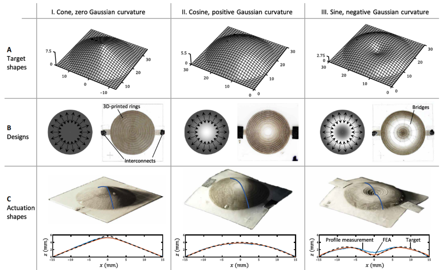
The cone, cosine, and sinusoidal target shapes with zero, positive, and negative Gaussian curvatures, respectively. (A) The actuator designs for the three target shapes. The schematic on the left-hand side shows the needed continuous actuation field to generate the target shape exactly, in which the arrows and color intensity represent the direction of the locally uniaxial actuation and the continuous number of active layers ( 0 \rightarrow \infty ), respectively. The images on the right-hand side show the fabricated DEAs approximating these deformation fields using 10 concentric stiff rings and 11 designed electrodes (12 total layers including two protective outer layers), in which the shade of gray represents the number of overlapping CNT electrodes, and the actuation direction is locally normal to the rings. (B) The actuation shapes for the three actuators. The images on the top are photographs of the actuated DEAs and the graphs on the bottom compare the cross-section of the actuation profiles (blue solid lines) to the target shapes (black dashed lines) and FEA (orange solid lines).
