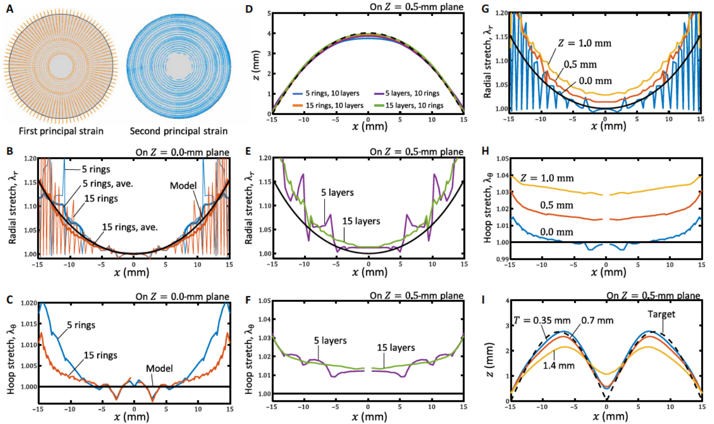
Figure 1. (A) For a DEA with five rings and 10 layers, designed to morph into the spherical cap of Fig. 1, the first and second principal strains are directed along the radial and hoop directions, respectively. (B) For two DEAs morphing into the spherical cap using 5 and 15 rings, both with 10 layers and a total thickness of 1 mm, the radial stretch is similar, better seen using the smoothed moving average curves, averaged over 10% of the diameter. (C) The required unity hoop stretch is better reproduced for the higher number of rings. (D) Actuation profiles for DEAs with 5 and 15 rings, both with 10 layers, and with 5 and 15 layers, both with 10 rings, compared to the target shape (black dashed lines). (E) Comparing the radial actuation of two DEAs with 5 and 15 layers, both with 10 rings, shows jumps in radial stretch for the DEA with 5 layers and smooth changes in radial stretch for the DEA with 15 layers. (F) The hoop stretch for the two DEAs with 5 and 15 layers has a similar offset from the model. (G) The radial actuation of a DEA with 15 layers, 10 rings, and a thickness of 1 mm, morphing into the spherical cap, shows the increase in radial stretch at the midplane, z = 0.5 mm, and top plane, z = 1.0 mm, of the elastomer sheet, compared to the bottom plane, z = 0 , on which the stiff rings are deposited. (H) Similar to the radial stretch, the hoop stretch shifts away from the model as z increases. (I) Actuation profile of three DEAs, one with the same thickness as the DEA in Fig. 2 (column III), one with twice the thickness, and one with half the thickness.
