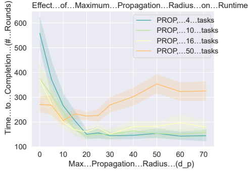
Figure 8: The effect of maximum propagation radius ( d_p ) on PROP completion time
