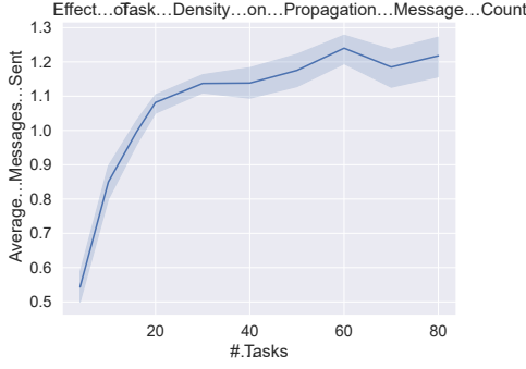
Figure 5: The effect of number of tasks on average messages sent per propagator agent per round (for PROP)
