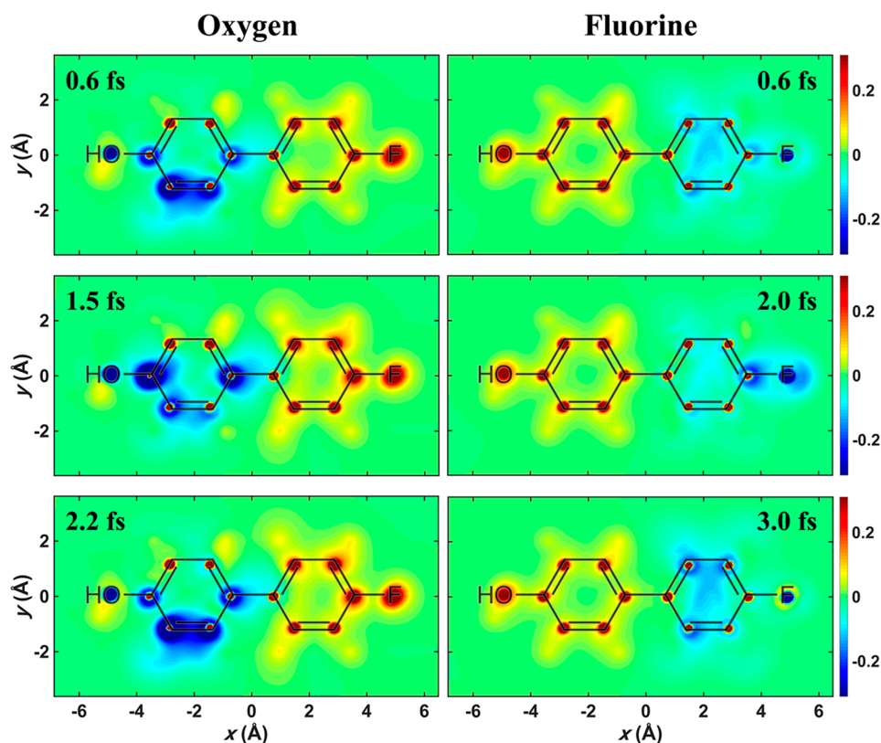
Figure 2. Snapshots of difference electronic charge density, \Delta\sigma_{\text{tot}}^E(\mathbf{r}, t) , in real space for the X-ray pump pulse tuned to the oxygen K-edge (left) and fluorine K-edge (right). The Cartesian coordinates are the same as in Figure 1. The charge densities are presented in the x - y plane by integrating over z .
