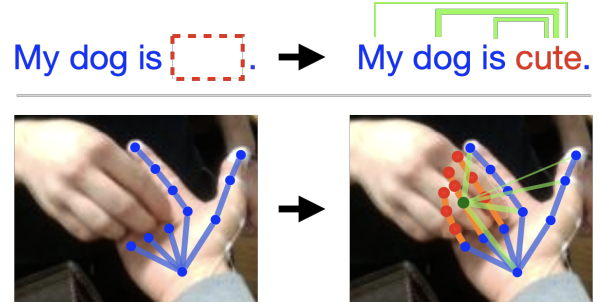
Fig. 1: Analogous to the fill-in-the-blank task that captures word correlations to predict blanked words ( Top ), PORT predicts occluded joints by capturing the semantic connectivity between hand joints ( Bottom ).
