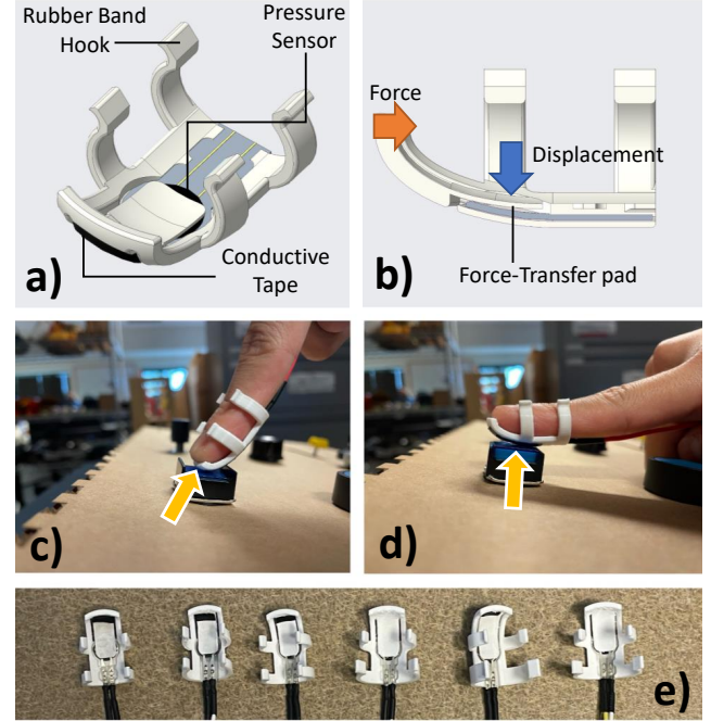
Figure 5: (a) CAD of the finger cap. (b c d) The force transfer pad allows the user to apply force through multiple angles. (e) The finger caps come in different sizes.
