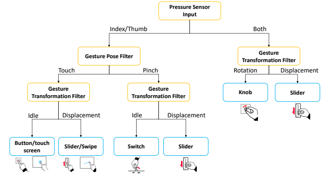
Figure 8: Decision Tree Algorithm.
